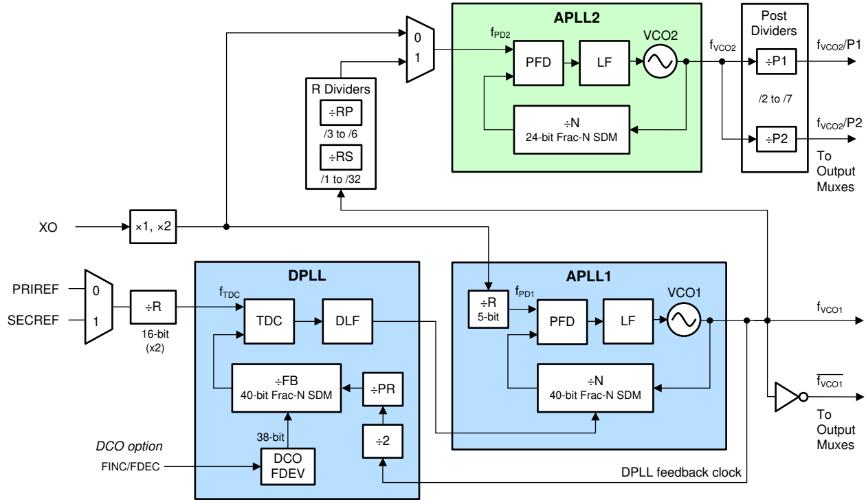
Figure 7-21. PLL Architecture
