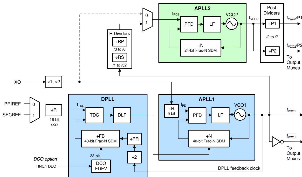
Figure 7-3. DPLL Mode With Cascaded APLL2
