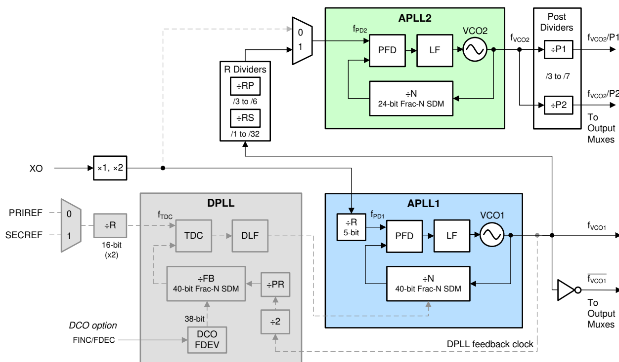
Figure 7-5. APLL-Only Mode With Cascaded APLL2
