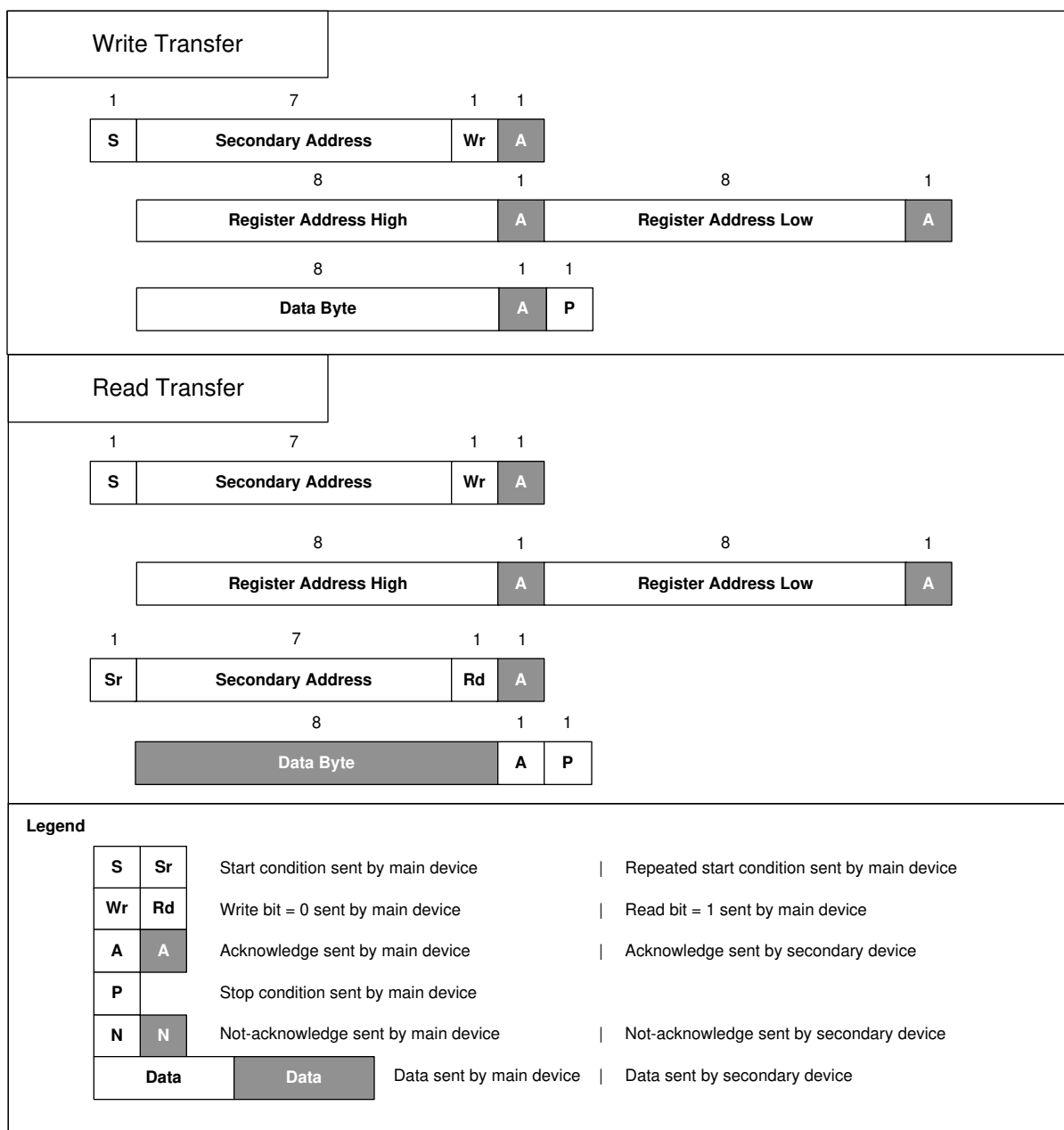
Figure 7-35. I 2 C Byte Write and Read Transfers
