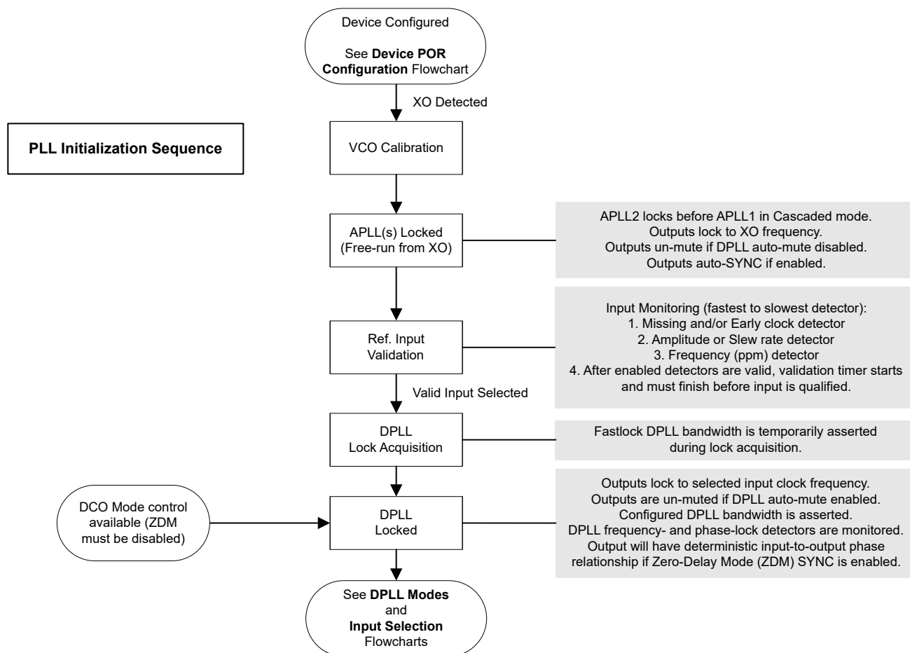
Figure 7-31. PLL Start-Up Sequence
