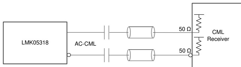
Figure 7-27. AC-CML Output to CML Receiver With Internal Termination/Biasing
