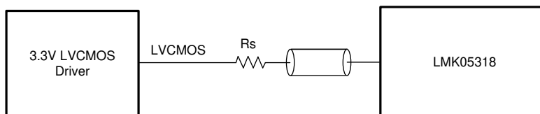
Figure 7-9. Single-Ended LVCMOS (1.8, 2.5, 3.3V) to Reference (PRIREF_P/SECREP_P)
