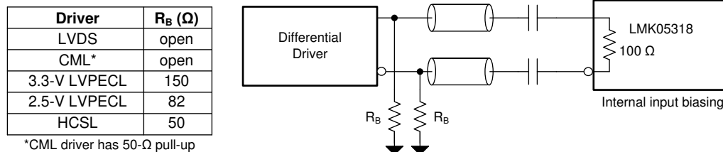
Figure 7-14. AC-Coupled Differential to Reference (PRIREF/SECREF) or XO Inputs
