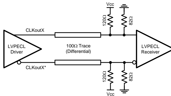
Figure 29. Differential LVPECL Operation, DC Coupling, Thevenin Equivalent
