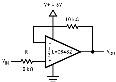
Figure 69. Half-Wave Rectifier with Input Current Protection (RI)
