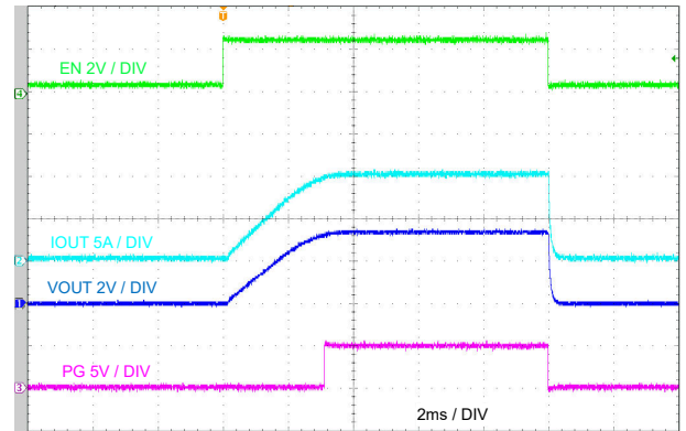
Figure 7-31. EN Start-Up and Shutdown Characteristic
