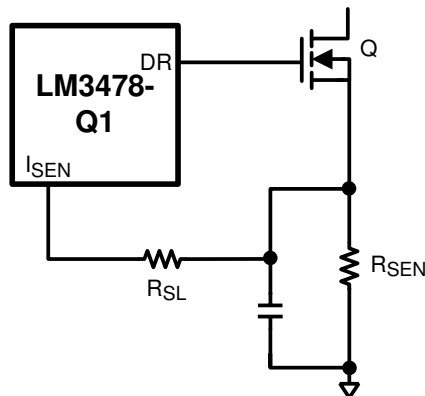
Copyright © 2017, Texas Instruments Incorporated Figure 6-4. Adding External Slope Compensation
