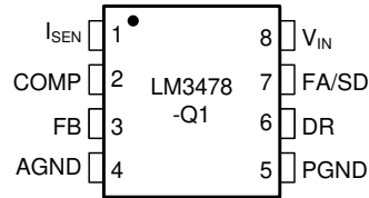
Figure 4-1. LM3478-Q1 DQFN Package, VSSOP-8 (Top View)
