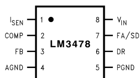
Figure 4-1. 8-Pin VSSOP (DGK) Package (Top View)
