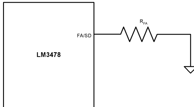
Figure 6-6. Frequency Adjust
