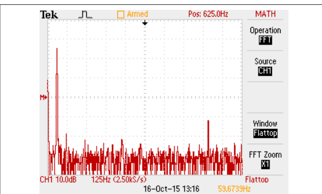
Figure 7-5. FFT of Signal in Previous Figure Shows Both the 60Hz Common-mode Along With 5kHz Differential Signal
