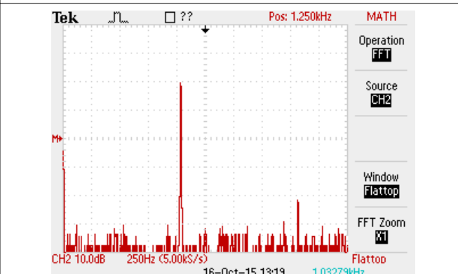
Figure 7-7. FFT of the INA126 Output Shows that the 60Hz Common-mode Signal is Rejected
