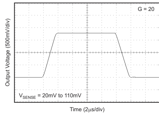
Figure 6-13. Step Response
