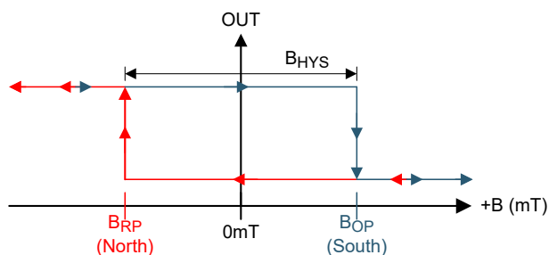
Figure 6-2. Output State (FA, AD, AG, BC Versions) Figure 6-3. Inverted Output State (ND, FD Versions)
