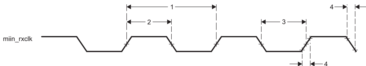
Figure 7-52. Clock Timing (GMAC Receive) - MII n operation
