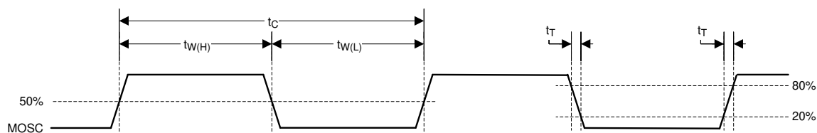
Figure 6-5. System Oscillators
