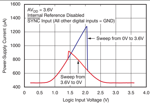
Figure 70. Power-Supply Current vs Logic Input Voltage
