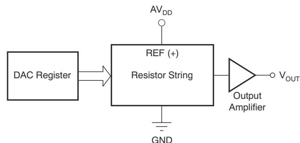
Figure 8-1. DACx311 Architecture
