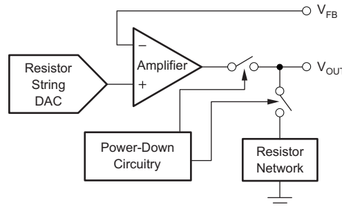
Figure 29. Output Stage During Power Down
