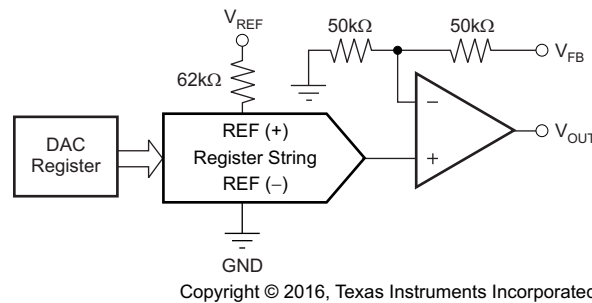
Figure 27. DACx551-Q1 Architecture
