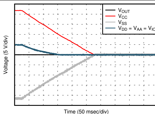
Figure 5-37. Power-Down Response
