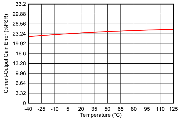
Figure 5-36. Current Output Gain Error vs Temperature
