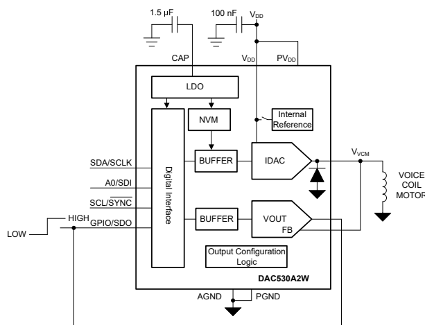
Voice Coil Motor Control Using the DAC530A2W
