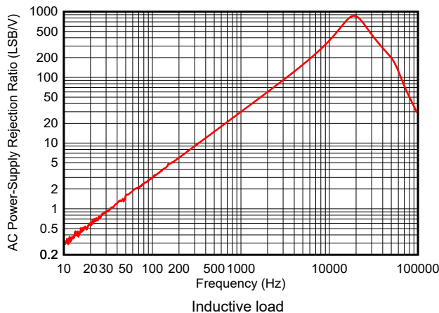
Inductive load
