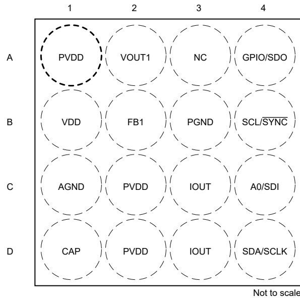
Figure 4-2. DAC530A2W: YBH Package, 16-Pin DSBGA (Top View)
