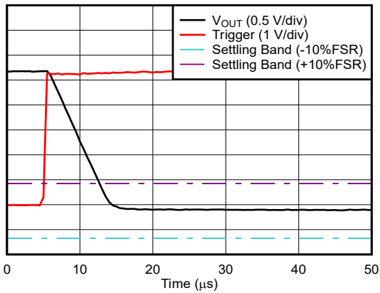
Full scale to zero scale swing
