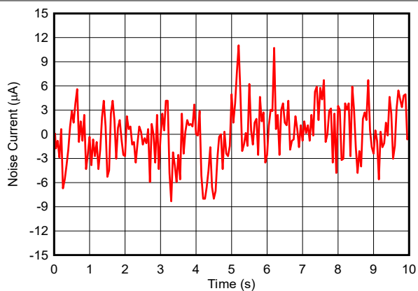
f = 0.1 Hz to 10 Hz, inductive load
