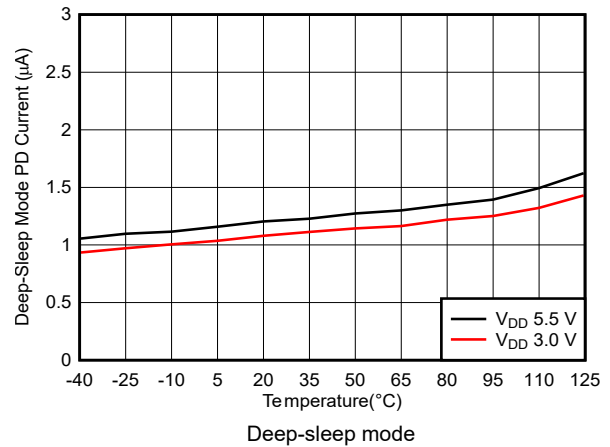
Figure 5-56. Power-Down Current vs Temperature
