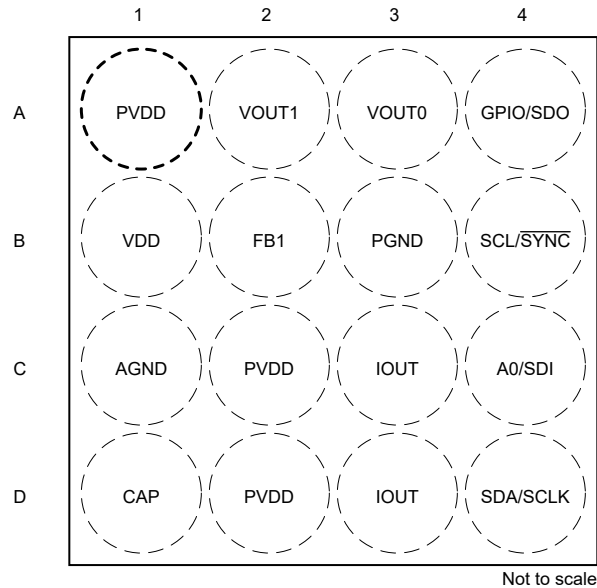
Figure 4-1. DAC532A3W: YBH Package, 16-Pin DSBGA (Top View)
