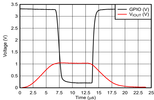
Figure 8-3. Comparator Toggle
