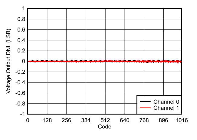
Figure 5-9. Voltage Output DNL vs Digital Input Code
