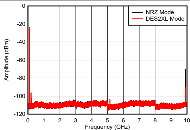
10MHz tone spacing, includes PCB, cable and balun loss Figure 6-39. Dual Tone, f_{\text{OUT}} = 97\text{MHz} , -6dBFS (0 - f_{\text{CLK}} )
