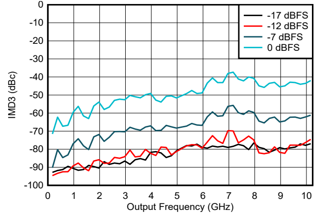
Figure 6-135. IMD3 vs Frequency and Digital Amplitude in NRZ/RF Modes
