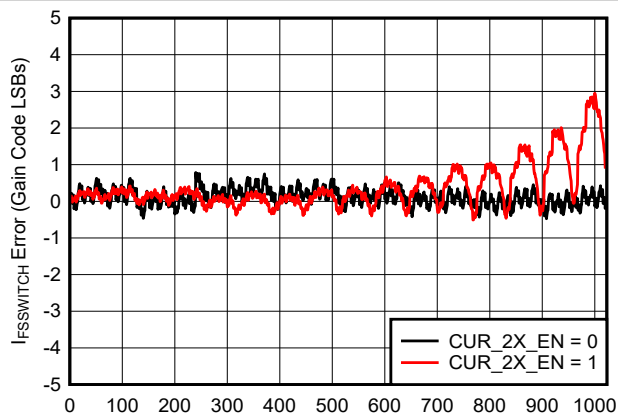
Figure 6-15. I_{\text{FS\_SWITCH}} vs Gain Code
