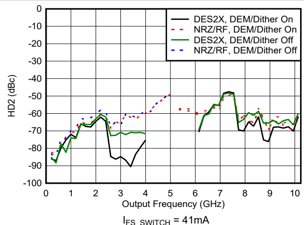
Figure 6-109. HD2 vs Frequency and Mode
