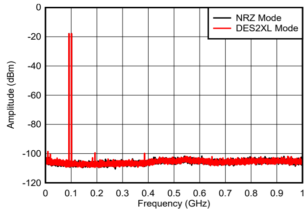
10MHz tone spacing, includes PCB, cable and balun loss Figure 6-38. Dual Tone, f_{\text{OUT}} = 97\text{MHz} , 0dBFS (0 - 1GHz)
