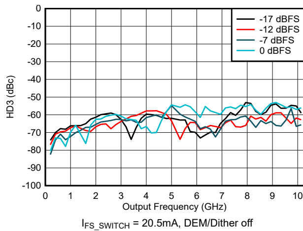
Figure 6-176. HD3 vs Frequency and Digital Amplitude in NRZ/RF Modes
