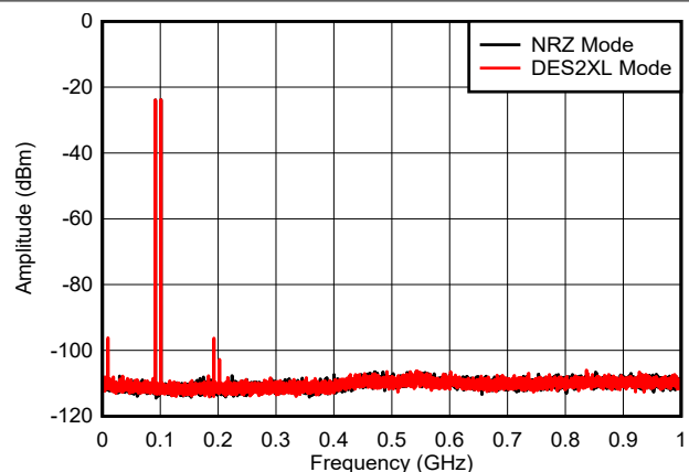
10MHz tone spacing, includes PCB, cable and balun loss Figure 6-40. Dual Tone, f_{\text{OUT}} = 97\text{MHz} , -6dBFS (0 - 1GHz)
