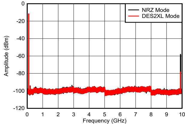
10MHz tone spacing, includes PCB, cable and balun loss Figure 6-37. Dual Tone, f_{\text{OUT}} = 97\text{MHz} , 0dBFS (0 - f_{\text{CLK}} )
