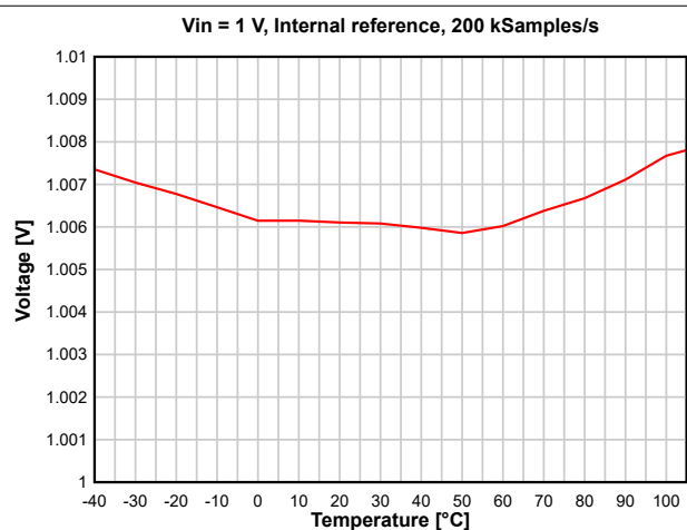
Figure 8-26. ADC Accuracy versus Temperature
