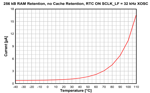
Figure 7-4. Standby Mode (MCU) Current vs. Temperature
