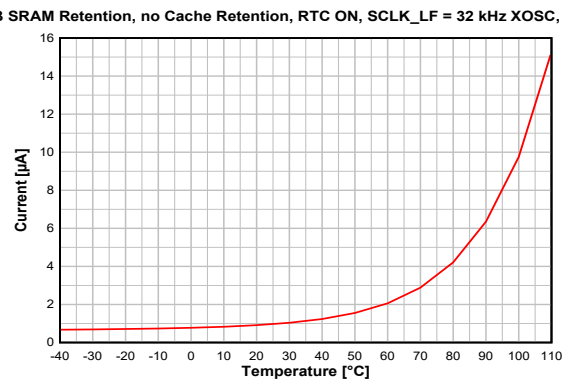
Figure 7-5. Standby Mode (MCU) Current vs. Temperature (VDD = 3.6V)
