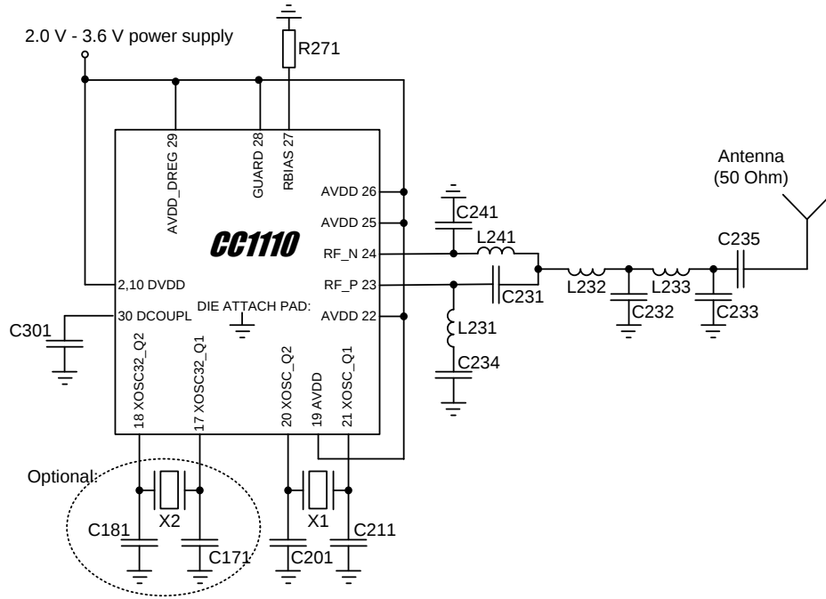
Figure 10: Application Circuit for CC110F 315/433 MHz (excluding supply decoupling capacitors)
