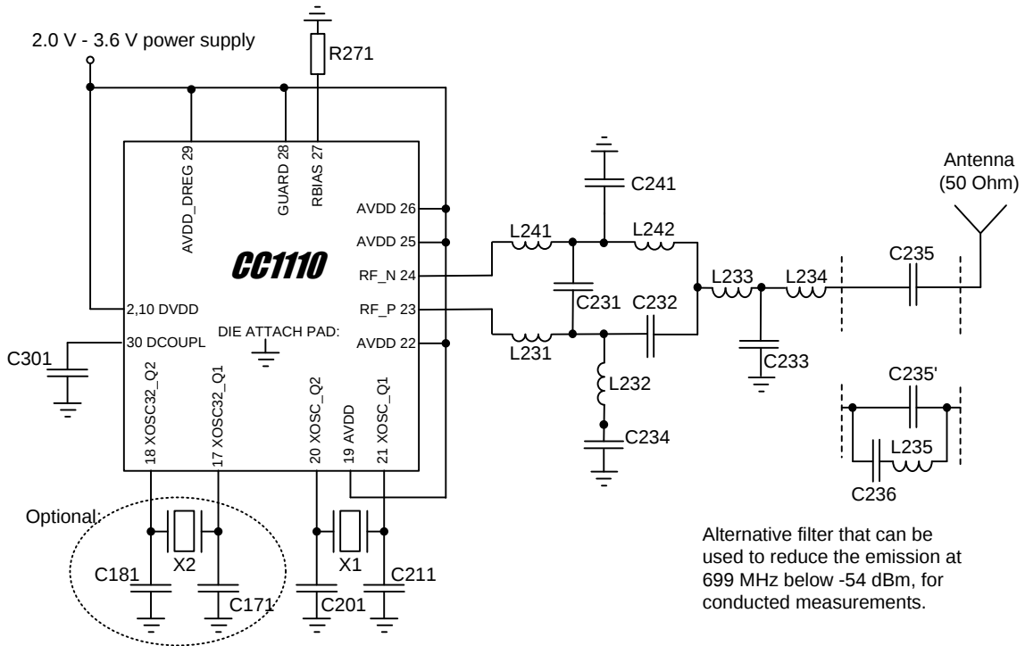
Figure 11: Application Circuit for CC110F 868/915 MHz (excluding supply decoupling capacitors)
