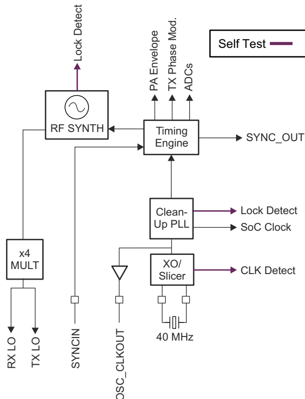
Figure 7-1. Clock Subsystem
