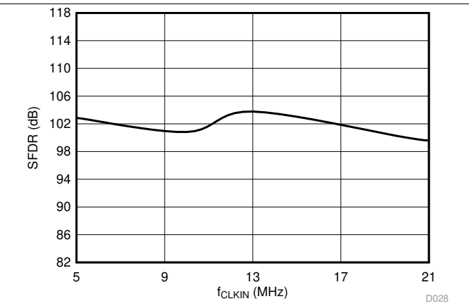
Figure 30. Spurious-Free Dynamic Range vs Clock Frequency
