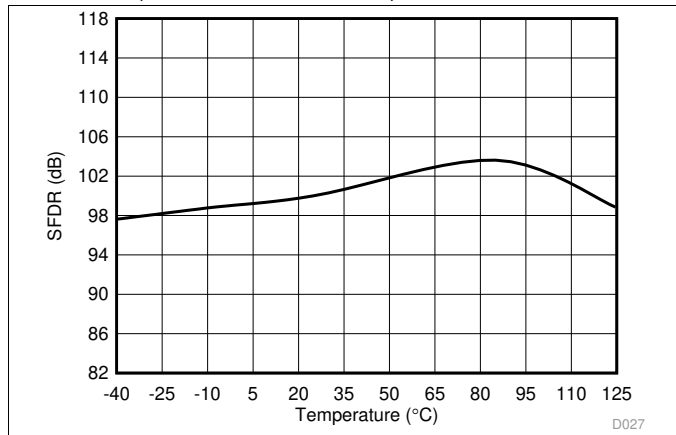
Figure 29. Spurious-Free Dynamic Range vs Temperature
