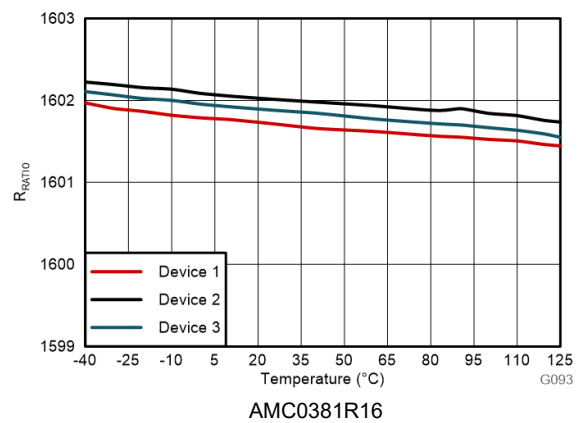
Figure 6-10. Divider Ratio vs Temperature
