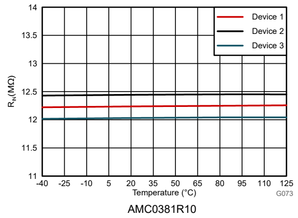
Figure 6-6. Input Resistance vs Temperature
