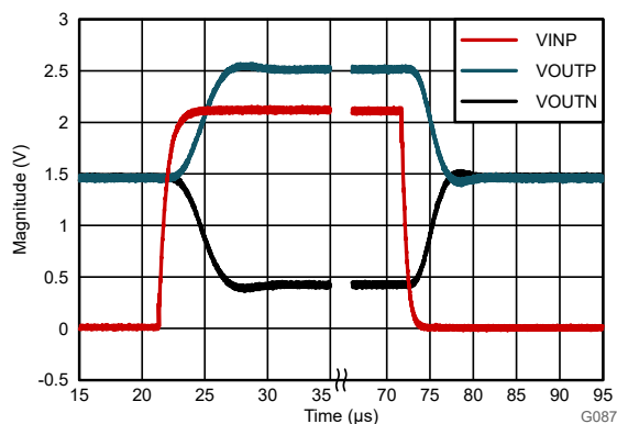
Figure 8-4. Step Response of the AMC0x11D
