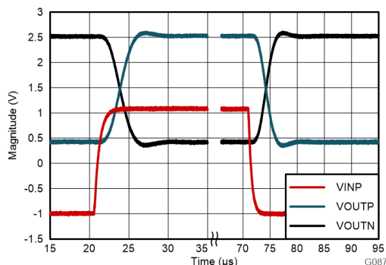
Figure 8-4. Step Response of the AMC0x30D-Q1
