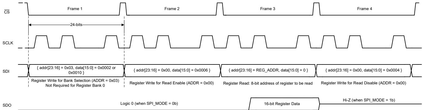
Figure 7-14. Register Read
