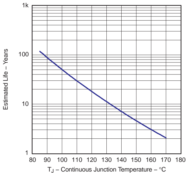
Figure 68. Operating Life Derating Chart, Electro Migration Fail Mode
