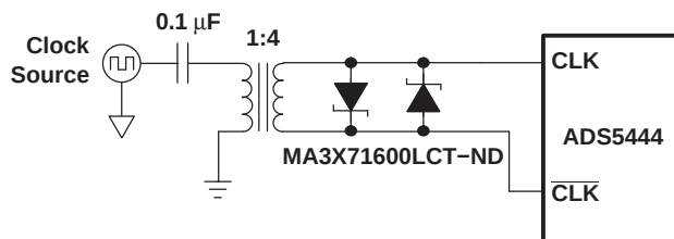
Figure 17. Differential Clock
