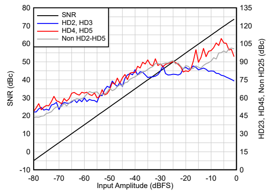
Figure 6-14. AC Performance vs A_{IN}
