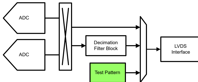
Figure 8-66. Test Pattern Generator
