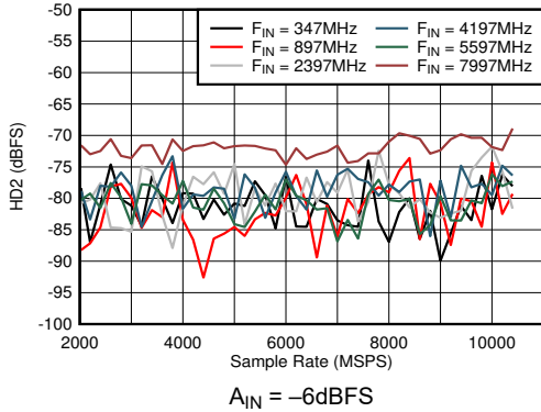
Figure 5-37. DES Mode: HD2 vs Sample Rate and Input Frequency A_{\text{IN}} = -6\text{dBFS}
