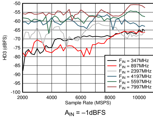
Figure 5-39. DES Mode: HD3 vs Sample Rate and Input Frequency A_{\text{IN}} = -1\text{dBFS}
