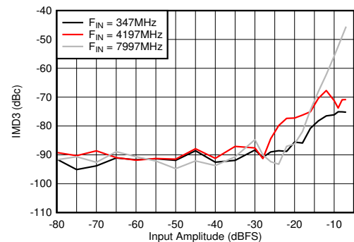
Figure 5-102. DES Mode: IMD3 vs Input Amplitude
