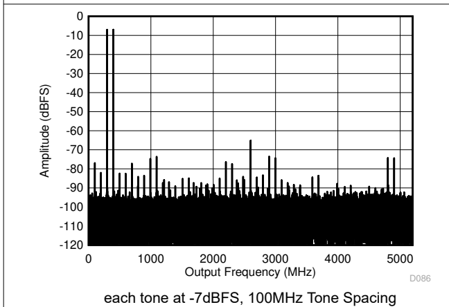
Figure 5-11. DES Mode: Two Tone FFT at 347MHz
