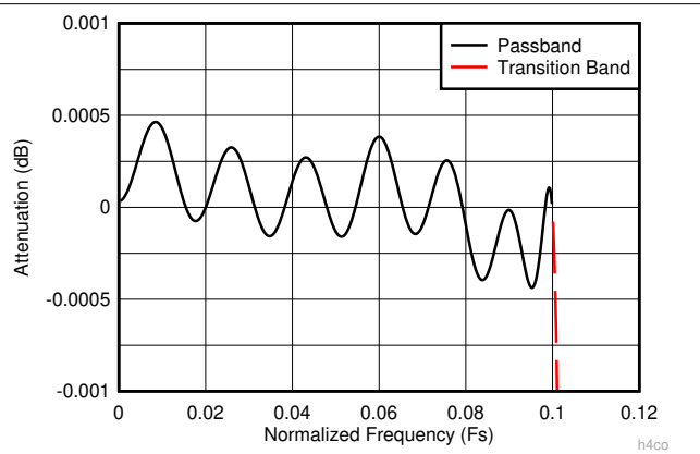
Figure 6-12. Decimate-by-4 Composite Zoomed Pass-Band Response
