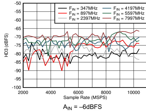
Figure 5-40. DES Mode: HD3 vs Sample Rate and Input Frequency A_{\text{IN}} = -6\text{dBFS}
