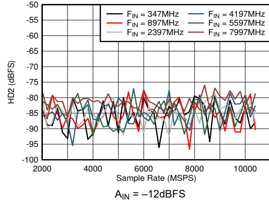
Figure 5-38. DES Mode: HD2 vs Sample Rate and Input Frequency A_{\text{IN}} = -12\text{dBFS}
