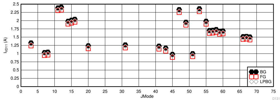
Figure 5-116. Dual Channel Mode: I_{VA11} vs JMODE at 5.2GSPS
