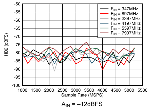
Figure 5-54. Dual Channel Mode: HD2 vs Sample Rate and Input Frequency
