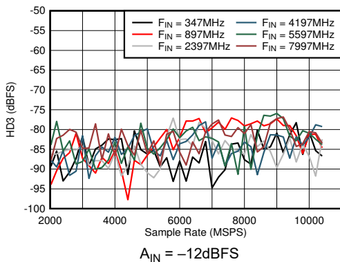
Figure 5-41. DES Mode: HD3 vs Sample Rate and Input Frequency A_{\text{IN}} = -12\text{dBFS}
