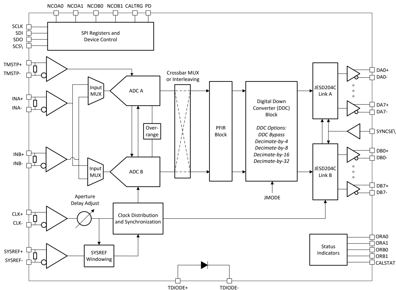
Block Diagram
