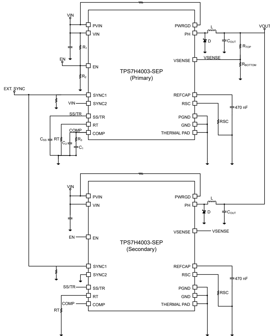
图 8-3. Parallel Configuration With External Sync
