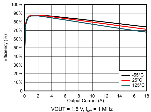
FIG 6-36. Efficiency for VIN = 3 V
