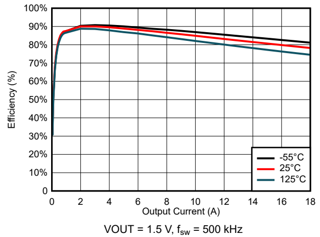
FIG 6-26. Efficiency for VIN = 5 V
