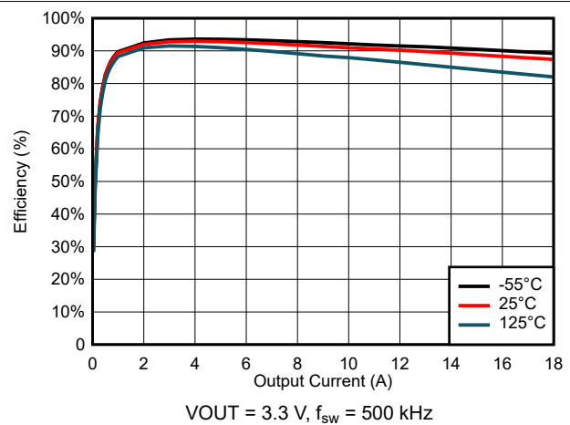
FIG 6-34. Efficiency for VIN = 7 V
