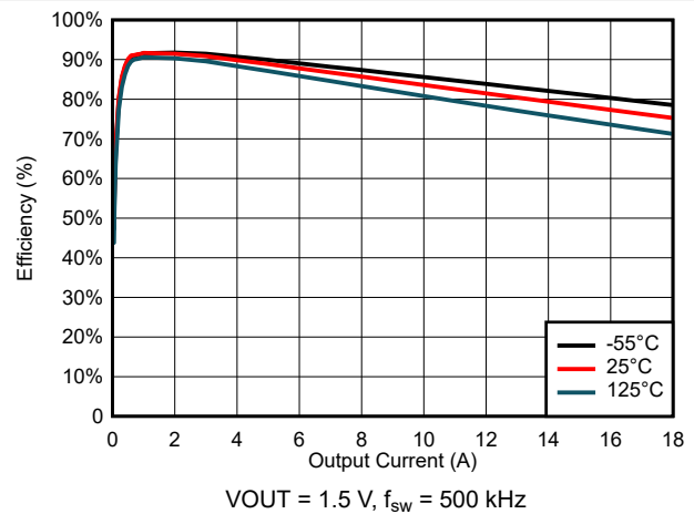
Figure 6-22. Efficiency for V_{IN} = 3\text{ V}
