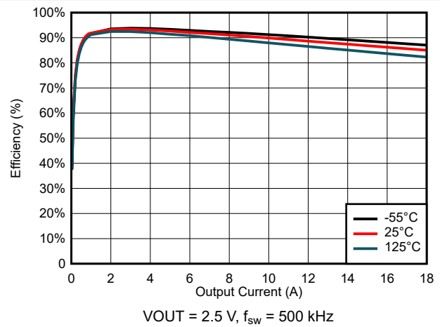
FIG 6-28. Efficiency for VIN = 5 V
