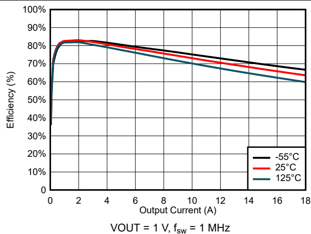
FIG 6-35. Efficiency for VIN = 3 V
