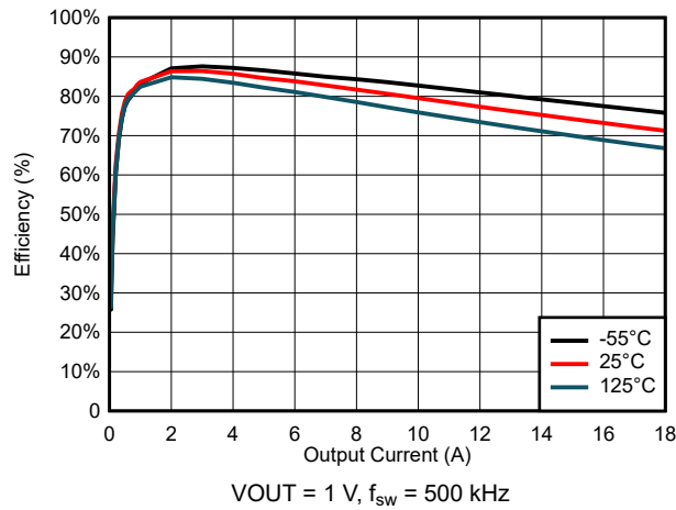
FIG 6-25. Efficiency for VIN = 5 V
