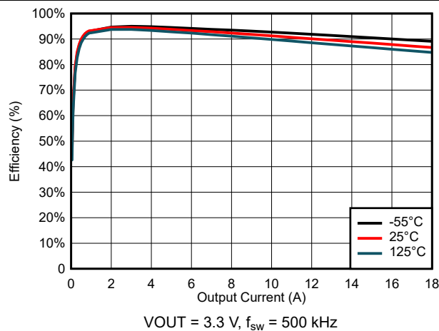
FIG 6-29. Efficiency for VIN = 5 V
