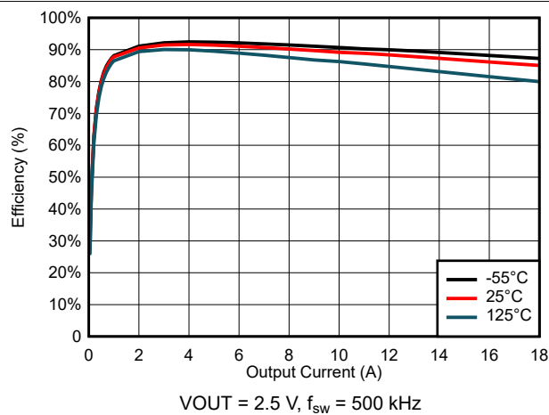
FIG 6-33. Efficiency for VIN = 7 V
