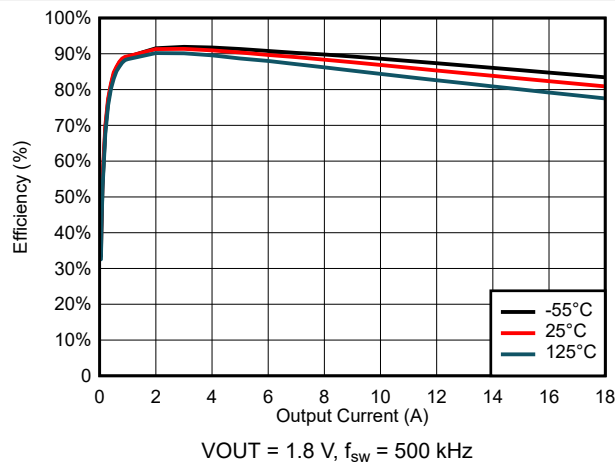
FIG 6-27. Efficiency for VIN = 5 V
