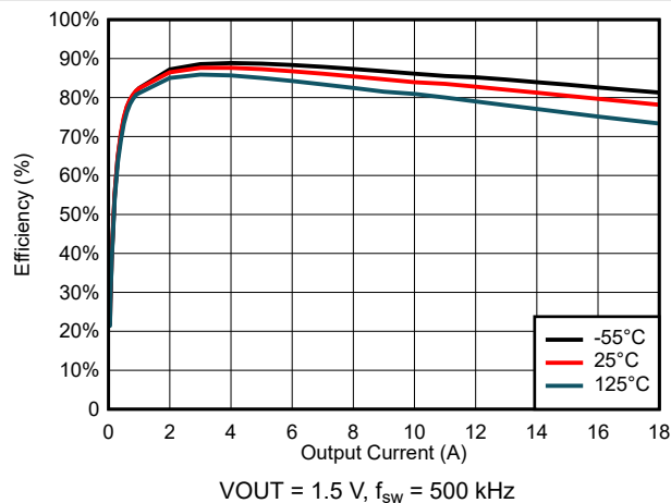
FIG 6-31. Efficiency for VIN = 7 V
