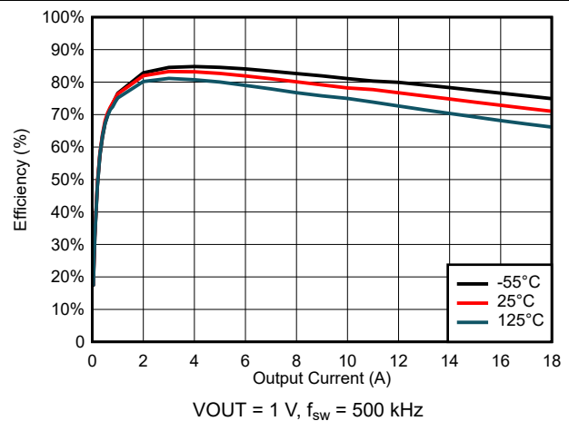
FIG 6-30. Efficiency for VIN = 7 V
