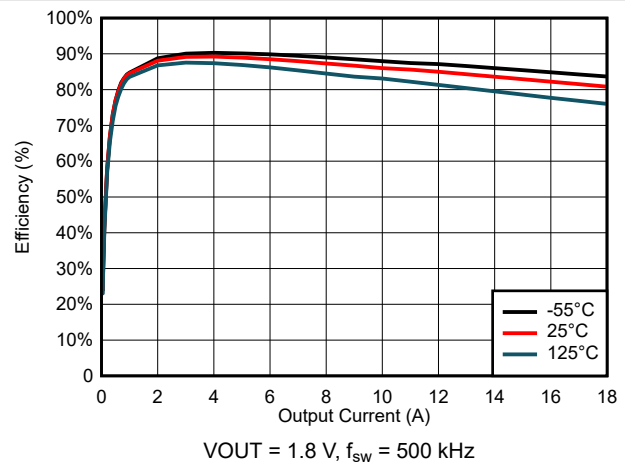
FIG 6-32. Efficiency for VIN = 7 V
