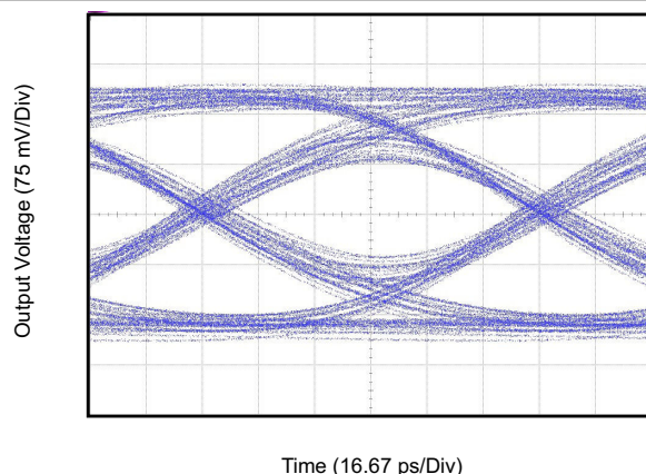
Figure 6-10. USB 3.1 Gen2 Eye-Pattern Performance with 12-inch Input PCB Trace at 10 Gbps
