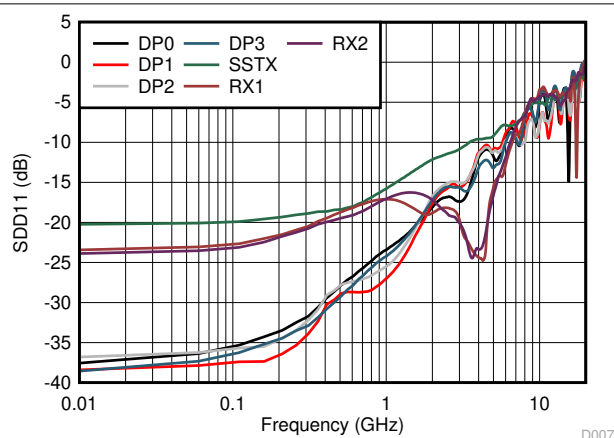
Figure 6-7. Input Return Loss Performance
