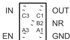
図 4-3. YZQ Package, 5-Pin DSBGA (Top View) (Legacy Chip Only)
