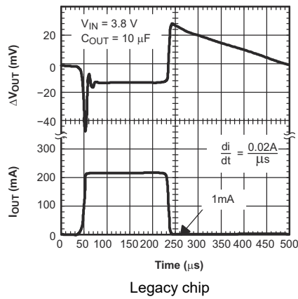
FIG 5-25. TPS79328 Load Transient Response
