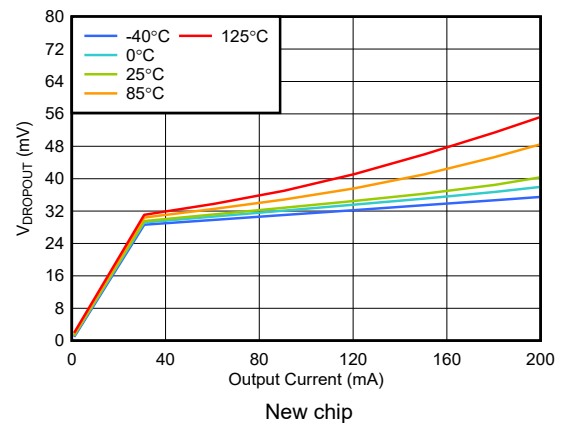
FIG 5-30. Dropout Voltage vs Output Current
