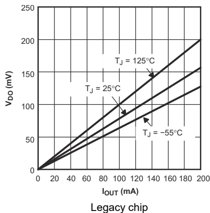
FIG 5-29. Dropout Voltage vs Output Current
