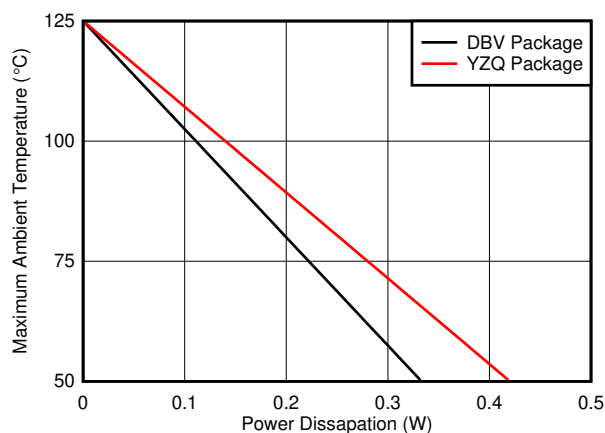
Figure 7-8. Maximum Ambient Temperature vs Power Dissipation
