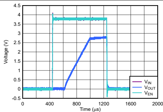
図 7-5. TPS79328 Output Voltage, Enable Voltage vs Time (Start-Up)
