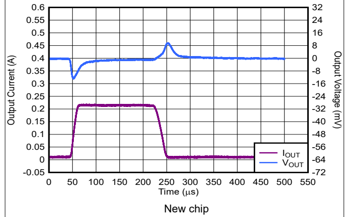
FIG 5-26. TPS79328 Load Transient Response
