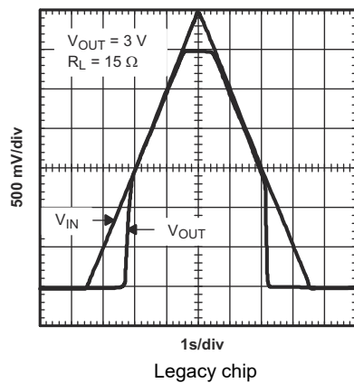
FIG 5-27. Power-Up and Power-Down
