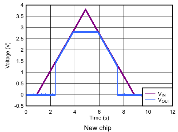
FIG 5-28. Power-Up and Power-Down
