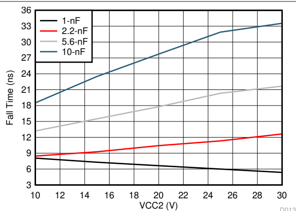
FIG 6-41. UCC5350SBD Fall Time vs C_L and V_{CC2}
