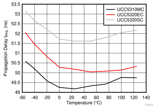
Figure 6-34. Propagation Delay t_{PHL} vs Temperature
