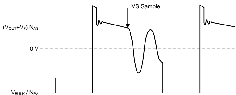
Figure 13. Auxiliary-Winding Voltage
