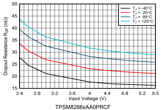
6-6. Dropout Resistance R DP
