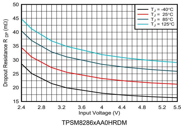
6-5. Dropout Resistance R DP
