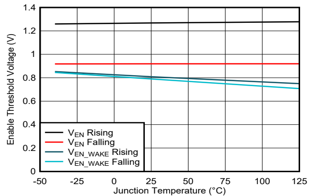
8-4. Enable Thresholds
