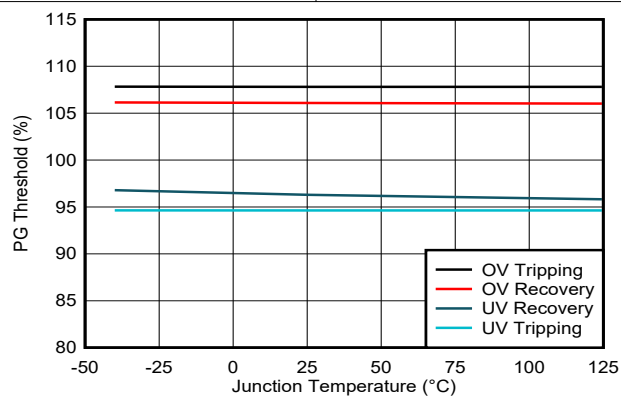
8-5. Power-Good (PG) Thresholds
