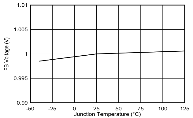
8-2. Feedback Voltage
