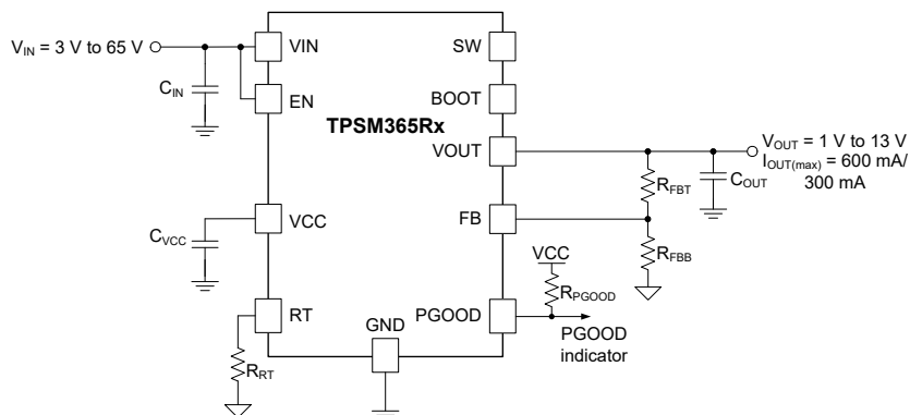
9-1. TPSM365Rx Schematic Diagram with Input Voltage Operating Range of 3 V to 65 V
