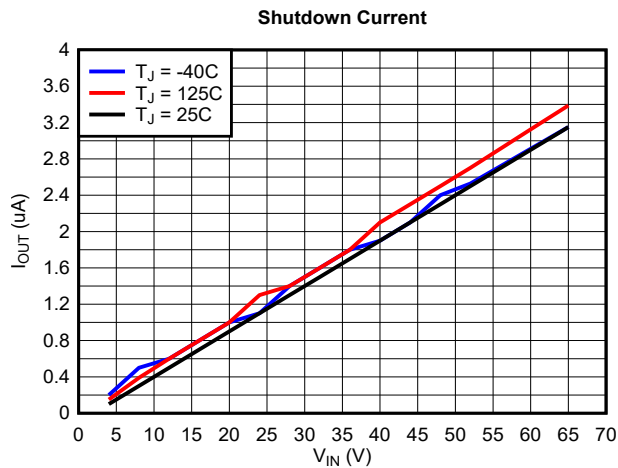
8-1. Shutdown Supply Current
