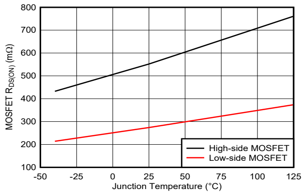
8-3. High-Side and Low-Side MOSFET R_{DS(on)}
