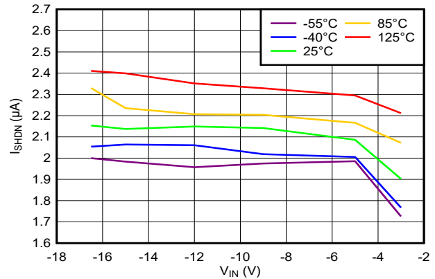
6-8. Shutdown Current vs Input Voltage Across Temperature
