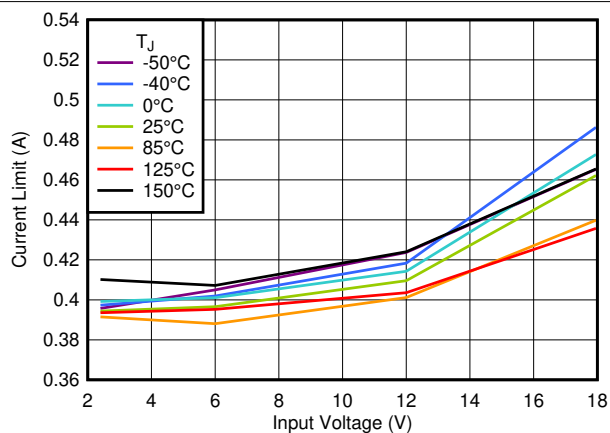
6-8. Current Limit vs V_{\text{IN}}
