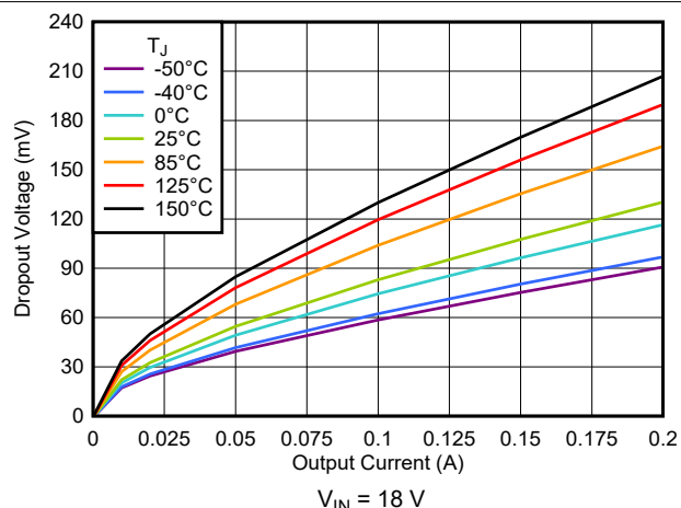
6-7. Dropout Voltage vs I_{\text{OUT}}
