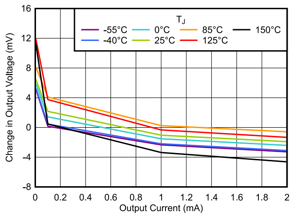
5-8. Load Regulation vs I_{OUT}
