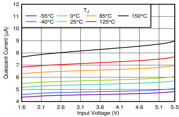
Figure 5-37. I_{GND} vs V_{IN} in the Dropout Region
