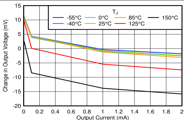
5-8. Load Regulation vs I_{OUT}
