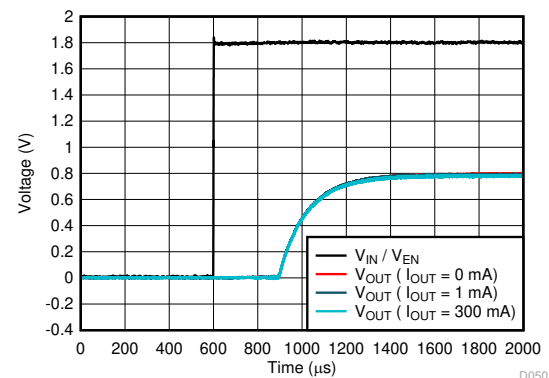
FIG 5-74. Start-Up
