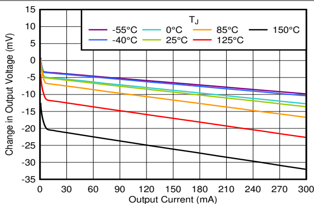
5-7. Load Regulation vs I_{OUT}
