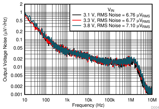
図 5-67. Noise vs Frequency and V_{IN}
