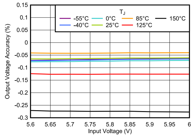
V_{OUT} = 5.5\text{ V} , V_{EN} = 1\text{ V} , DQN, YCJ, and YCK packages Figure 5-22. Output Voltage Accuracy vs V_{IN}
