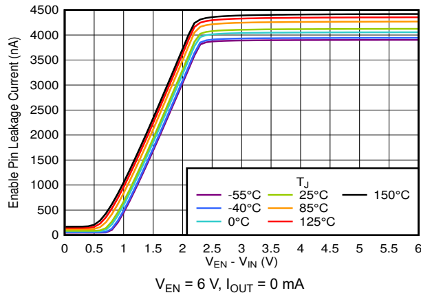
図 5-43. Enable Pin Leakage Current vs V_{EN} - V_{IN}
