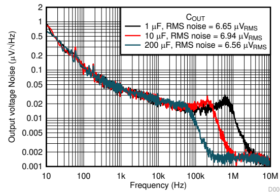
図 5-68. Noise vs Frequency and C_{OUT}
