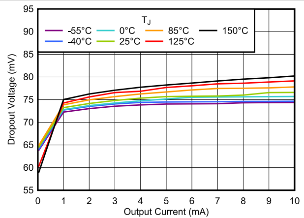
5-28. Dropout Voltage vs I_{OUT}
