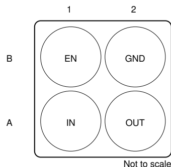
✎ 4-2. YCJ and YCK Packages, 4-Pin DSBGA (Bottom View)
