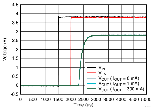
FIG 5-75. Start-Up
