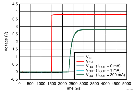
FIG 5-76. Start-Up
