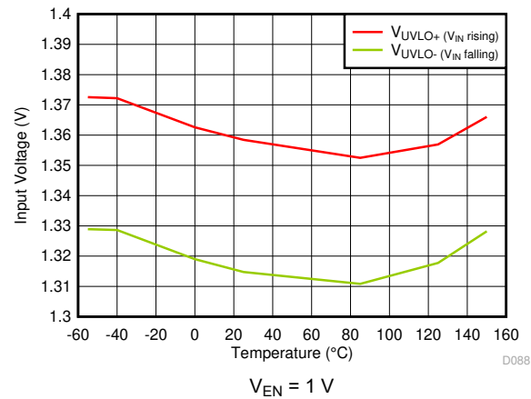
図 5-46. UVLO Threshold vs Temperature
