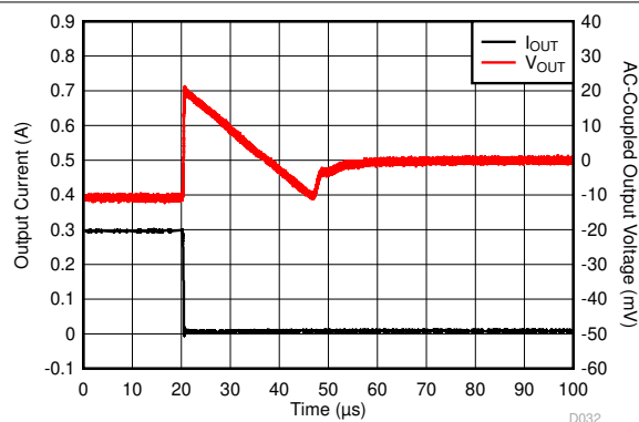
FIG 5-52. Load Transient
