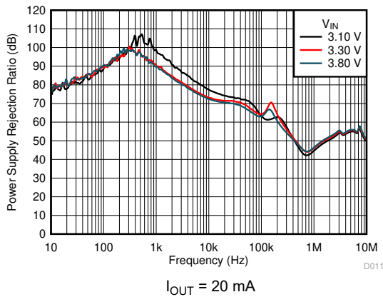
Figure 5-61. PSRR vs V_{IN} vs Frequency and V_{IN}
