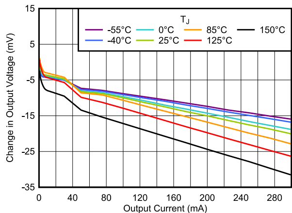
5-7. Load Regulation vs I_{OUT}
