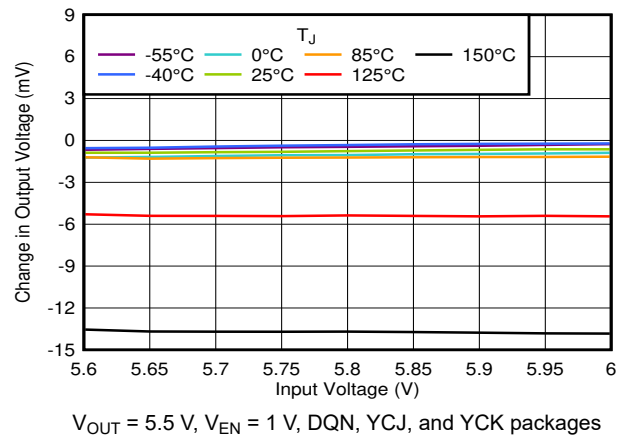
Figure 5-2. Line Regulation vs V_{IN}
