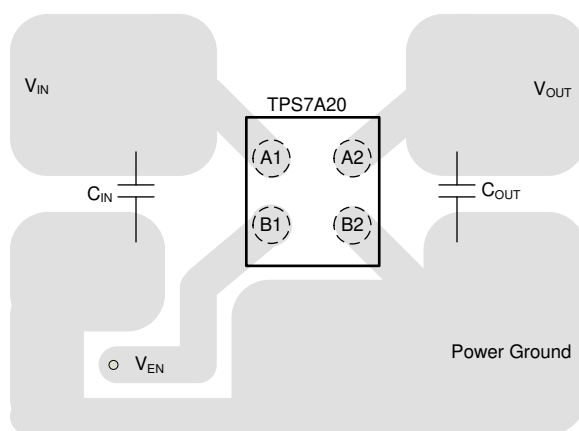
図 7-9. YCJ and YCK Package (DSBGA) Typical Layout
