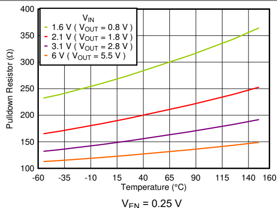
FIG 5-49. Output Pulldown Resistor vs Temperature
