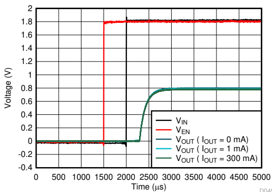
FIG 5-73. Start-Up Turn-On Time
