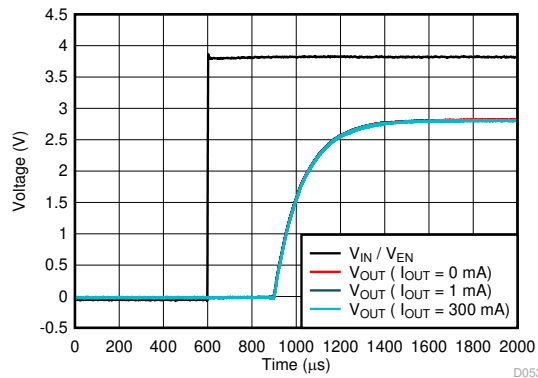
Figure 5-79. Start-Up
