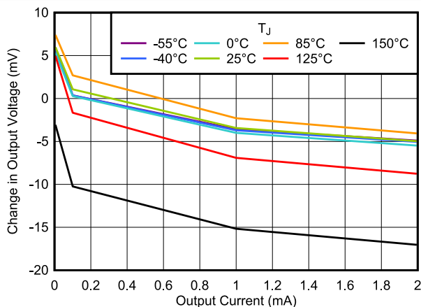
5-10. Load Regulation vs I_{OUT}
