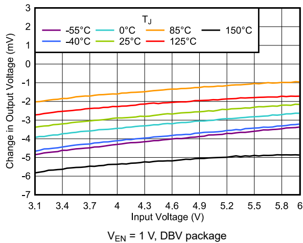
Figure 5-3. Line Regulation vs V_{IN}
