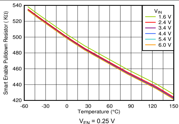
FIG 5-50. Smart Enable Pulldown Resistor vs Temperature and V_{IN}
