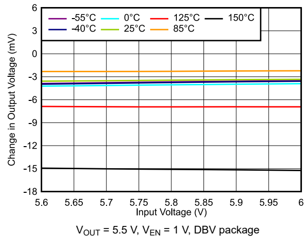
Figure 5-4. Line Regulation vs V_{IN}
