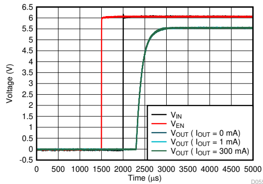
Figure 5-79. Start-Up
