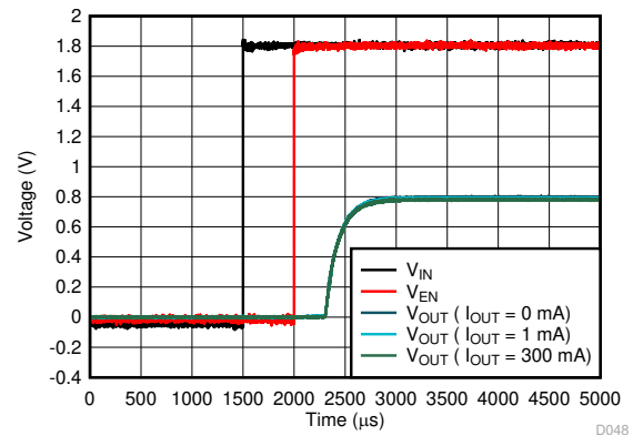
FIG 5-74. Start-Up
