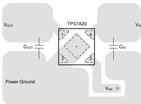
図 7-8. DQN Package (X2SON) Typical Layout
