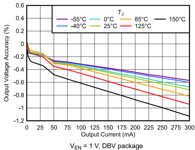
Figure 5-15. Output Voltage Accuracy vs I_{OUT}
