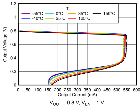
図 5-45. Current Limit
