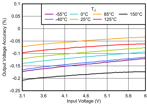
V_{EN} = 1\text{ V} , I_{OUT} = 1\text{ mA} , DQN, YCJ, and YCK packages Figure 5-21. Output Voltage Accuracy vs V_{IN}
