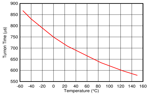
FIG 5-73. Start-Up Turn-On Time
