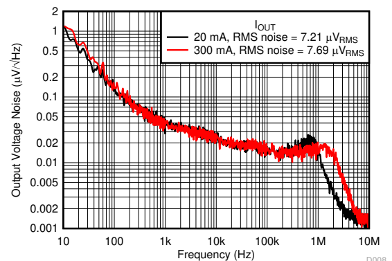
図 5-70. Noise vs Frequency and I_{OUT}
