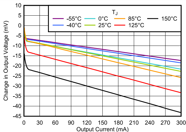
5-9. Load Regulation vs I_{OUT}
