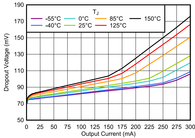
図 5-31. Dropout Voltage vs I_{OUT}
