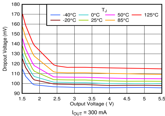
図 5-33. Dropout Voltage vs V_{OUT}
