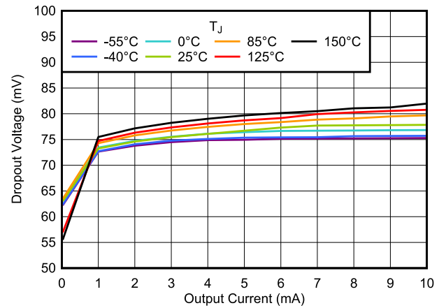
図 5-32. Dropout Voltage vs I_{OUT}
