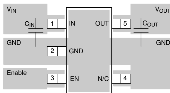
図 7-7. DBV Package (SOT-23) Typical Layout
