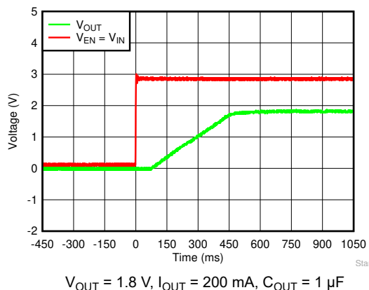
Figure 6-51. Startup With V_{EN} = V_{IN}
