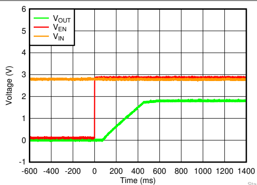
Figure 6-53. Startup With V_{EN} After V_{IN}
