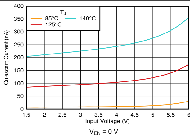
FIG 6-11. I_{SHDN} vs V_{IN} and Temperature
