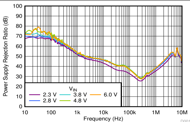
6-44. PSRR vs Frequency and V_{IN}
