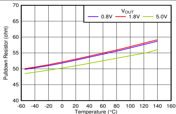
FIG 6-41. Pulldown Resistor vs Temperature and V_{OUT}
