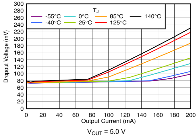
FIG 6-33. Dropout vs I_{OUT} and Temperature
