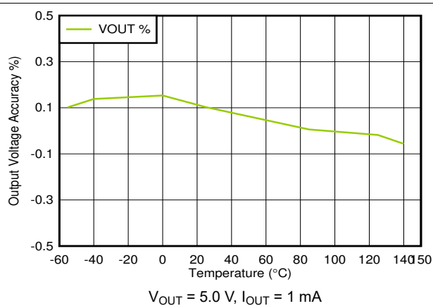
6-30. Output Accuracy vs Temperature
