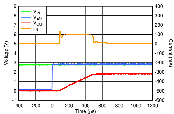
6-56. Startup Inrush Current With C_{OUT} = 22\text{ }\mu\text{F}
