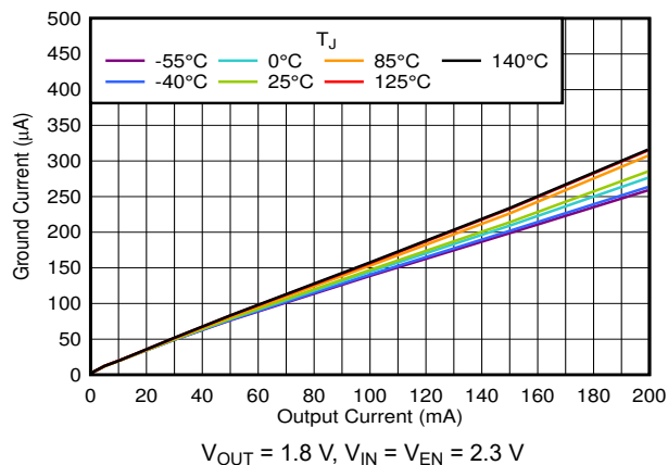
FIG 6-4. I_Q vs I_{OUT} and Temperature Up to 200 mA
