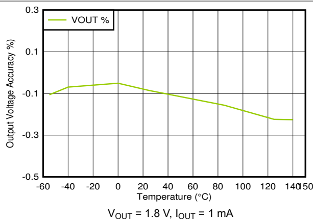
6-27. Output Accuracy vs Temperature
