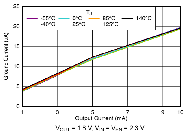
FIG 6-6. I_Q vs I_{OUT} and Temperature for 1 mA to 10 mA
