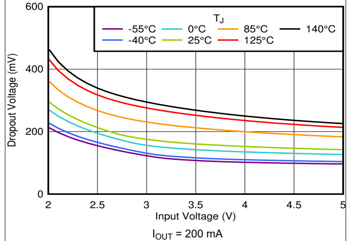
FIG 6-34. Dropout vs V_{IN} and Temperature
