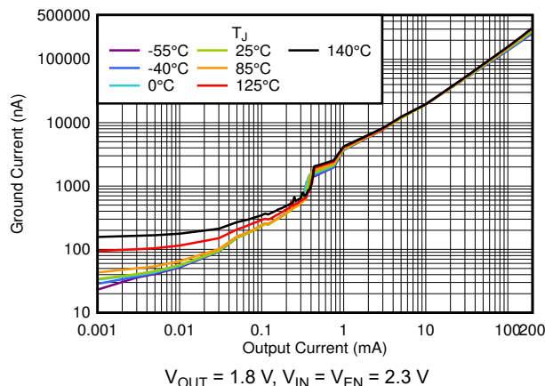
FIG 6-3. I_Q vs I_{OUT} and Temperature up to 200 mA
