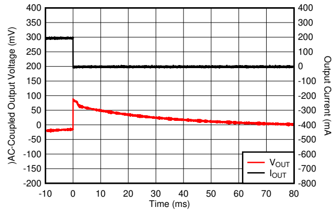
FIG 6-20. I_{OUT} Transient From 200 mA to 0 mA
