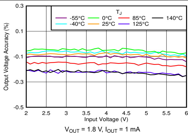
6-26. Output Accuracy vs V_{IN} and Temperature
