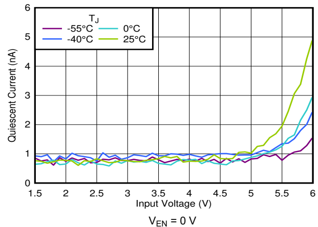
FIG 6-10. I_{SHDN} vs V_{IN} and Temperature
