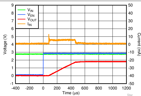
6-55. Startup Inrush Current With C_{OUT} = 1\text{ }\mu\text{F}
