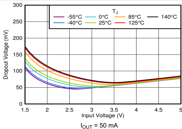
FIG 6-35. Dropout vs V_{IN} and Temperature
