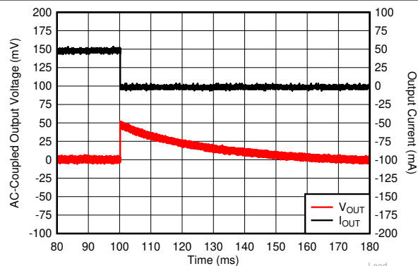
FIG 6-16. I_{OUT} Transient From 50 mA to 0 mA
