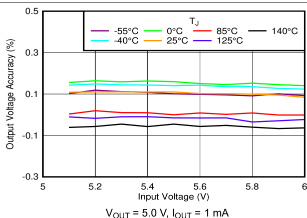
6-29. Output Accuracy vs V_{IN} and Temperature
