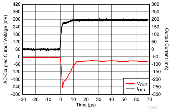
FIG 6-19. I_{OUT} Transient From 0 mA to 200 mA
