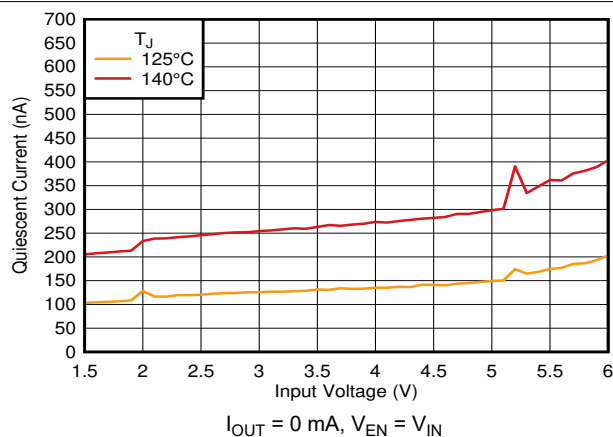
FIG 6-2. I_Q vs V_{IN} and Temperature
