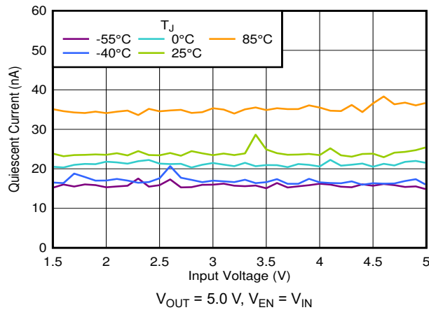
FIG 6-7. I_Q in Dropout vs V_{IN} and Temperature
