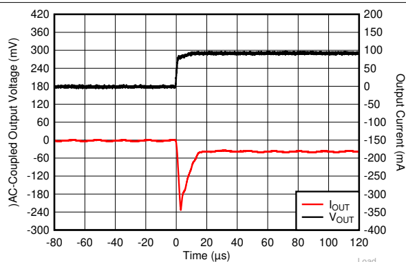
FIG 6-15. I_{OUT} Transient From 0 mA to 50 mA
