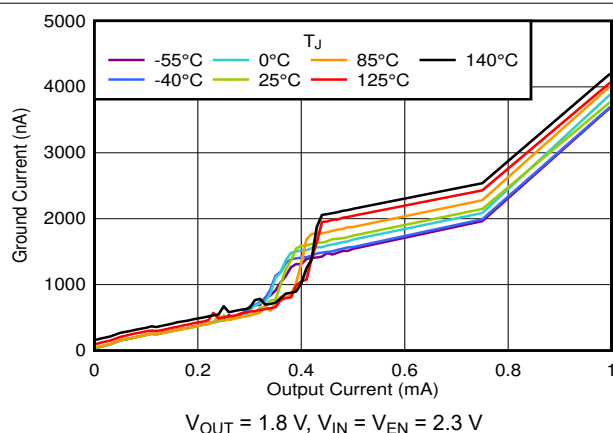
FIG 6-5. I_Q vs I_{OUT} and Temperature Up to 1 mA
