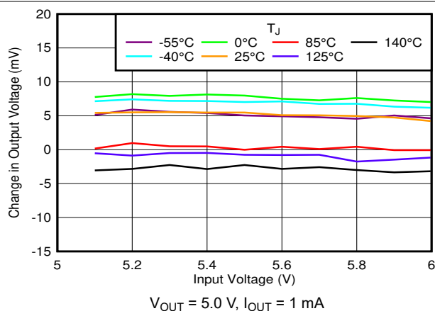
6-28. Line Regulation vs V_{IN} and Temperature
