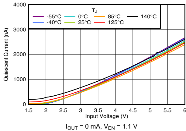
FIG 6-9. I_Q vs V_{IN} and Temperature
