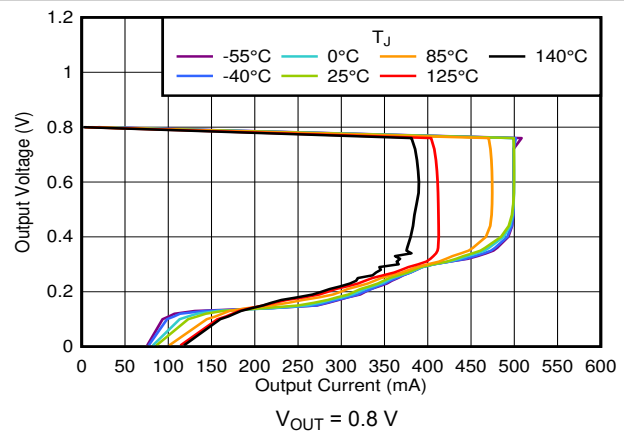
FIG 6-36. Foldback Current Limit vs I_{OUT} and Temperature
