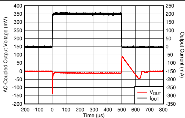
FIG 6-14. I_{OUT} Transient From 1 mA to 200 mA
