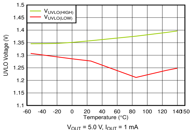
FIG 6-40. UVLO Rising and Falling Threshold vs Temperature
