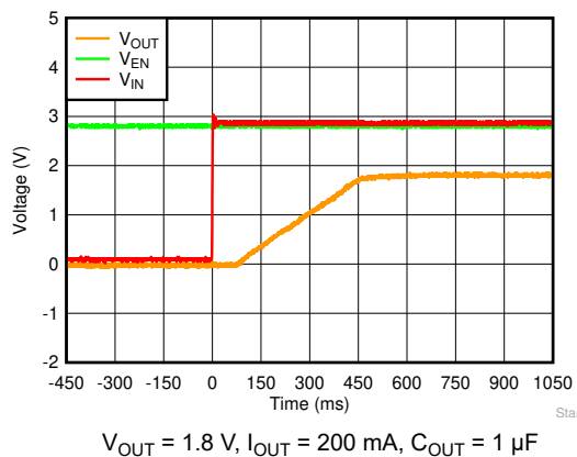
Figure 6-51. Startup With V_{EN} Before V_{IN}
