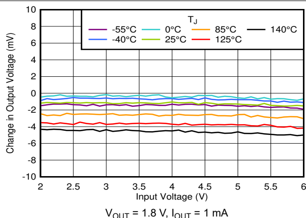
6-25. Line Regulation vs V_{IN} and Temperature
