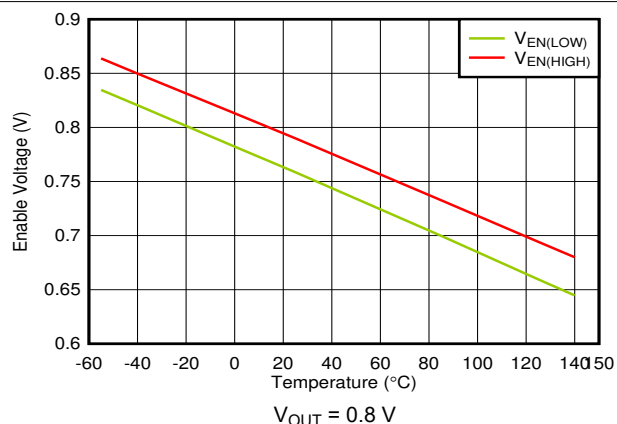
FIG 6-38. EN High and Low Threshold vs Temperature
