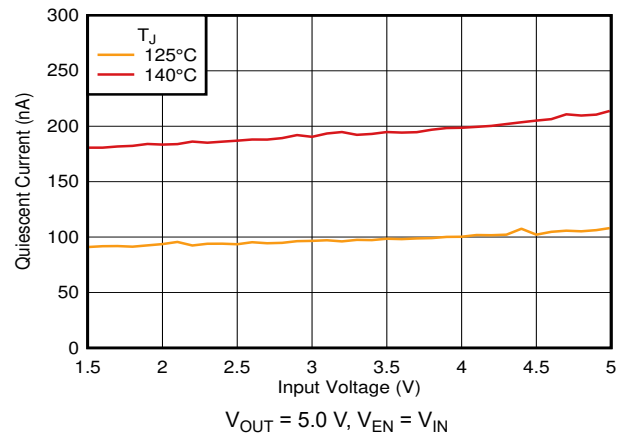
FIG 6-8. I_Q in Dropout vs V_{IN} and Temperature
