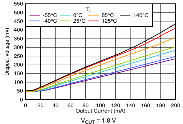
FIG 6-32. Dropout vs I_{OUT} and Temperature
