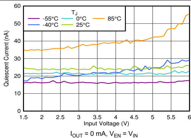
FIG 6-1. I_Q vs V_{IN} and Temperature
