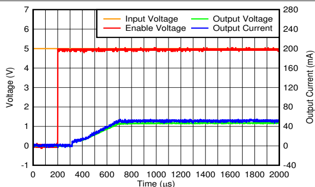
FIG 6-80. Start Up at 150^\circ\text{C}
