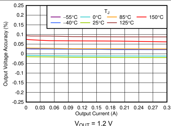
6-3. Output Accuracy vs I_{\text{OUT}}
