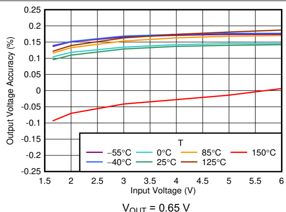
6-2. Output Accuracy vs V_{\text{IN}}
