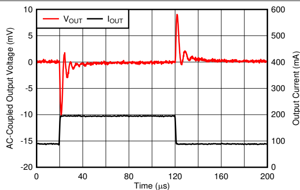
FIG 6-55. Load Transient
