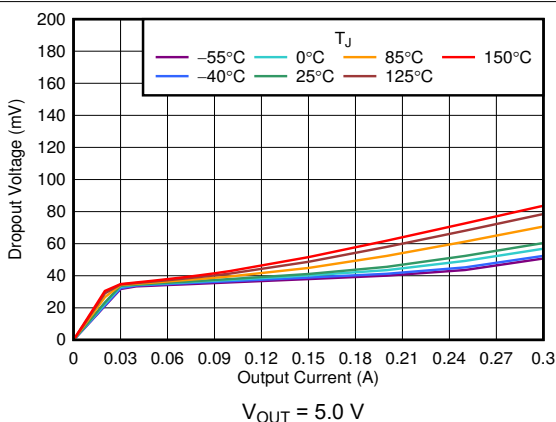
FIG 6-13. Dropout Voltage vs I_{OUT}
