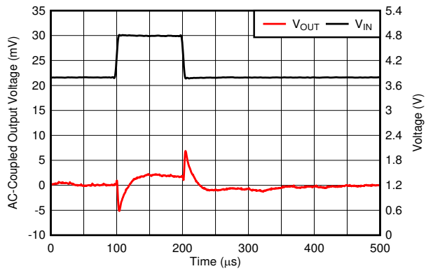
FIG 6-37. Line Transient
