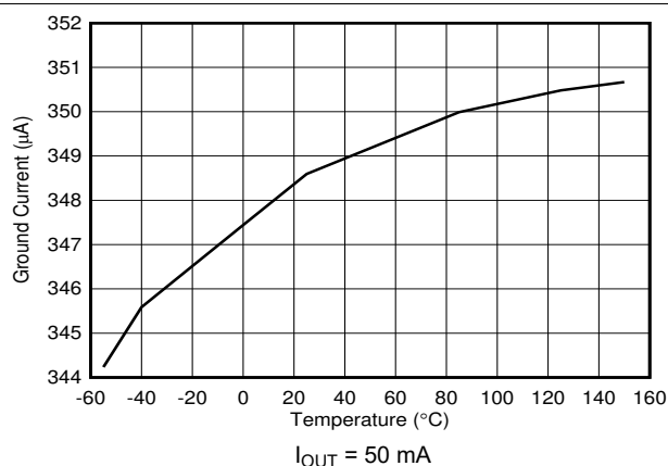
FIG 6-17. 50-mA Ground Current vs Temperature
