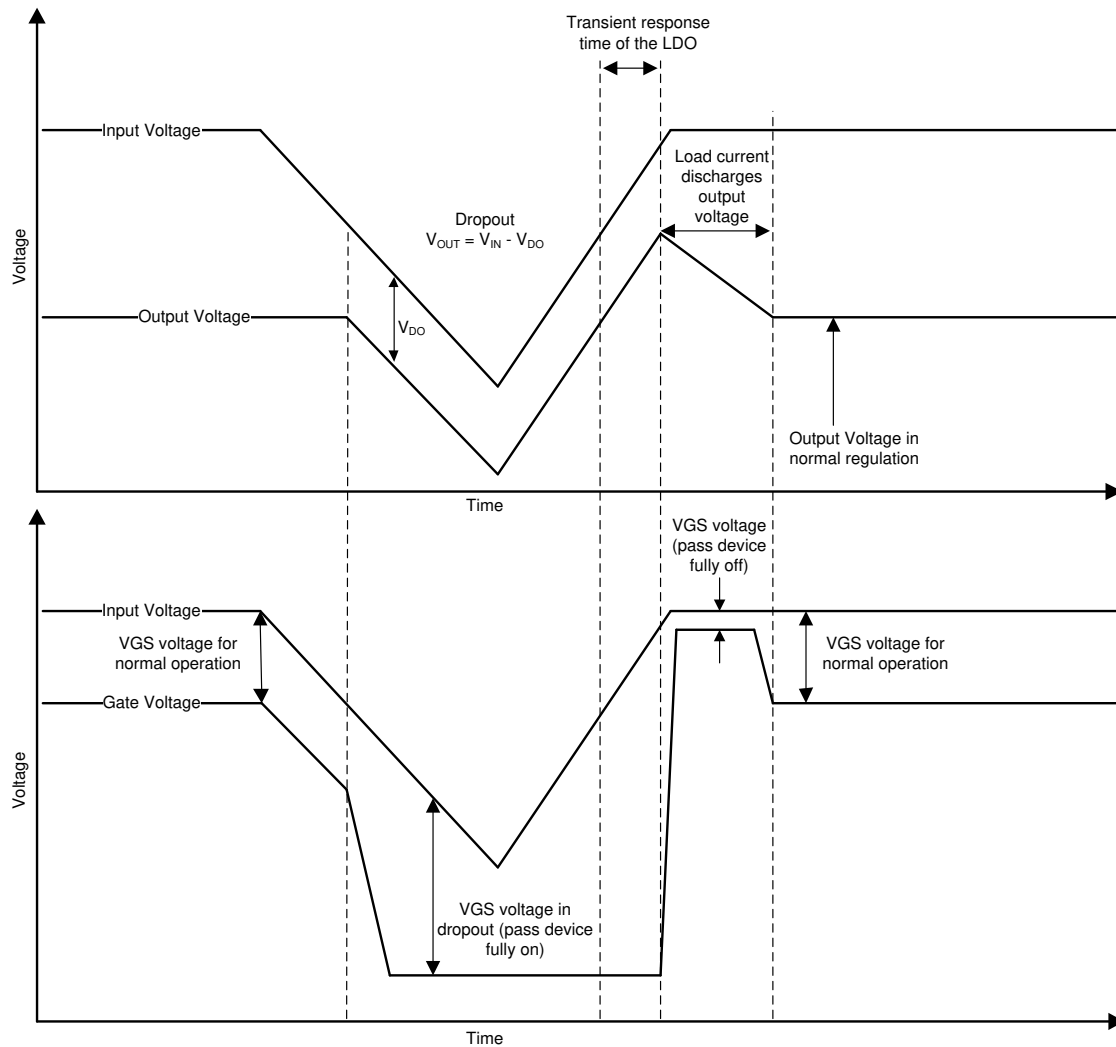
FIG 8-4. Line Transients From Dropout
