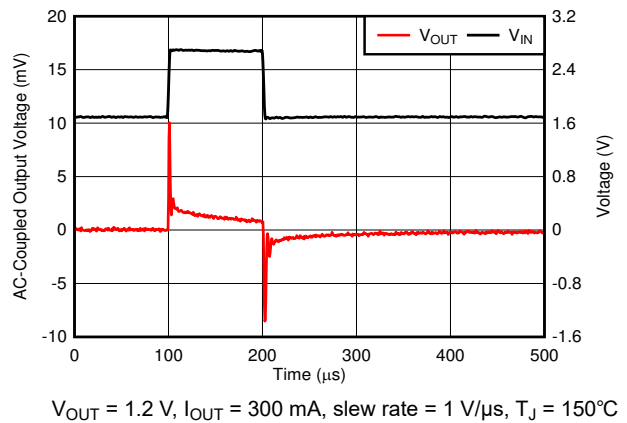
FIG 6-34. Line Transient
