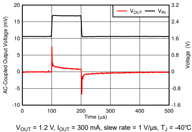
FIG 6-33. Line Transient
