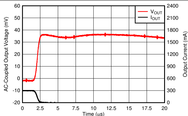
FIG 6-43. I_{OUT} Transient From 300 mA to 1 mA
