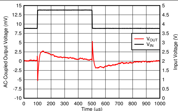
FIG 6-25. Line Transient
