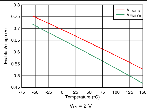
FIG 6-20. V_{EN(HI)} and V_{EN(LO)} Thresholds vs Temperature
