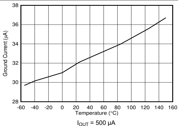
FIG 6-16. 500- \mu\text{A} Ground Current vs Temperature
