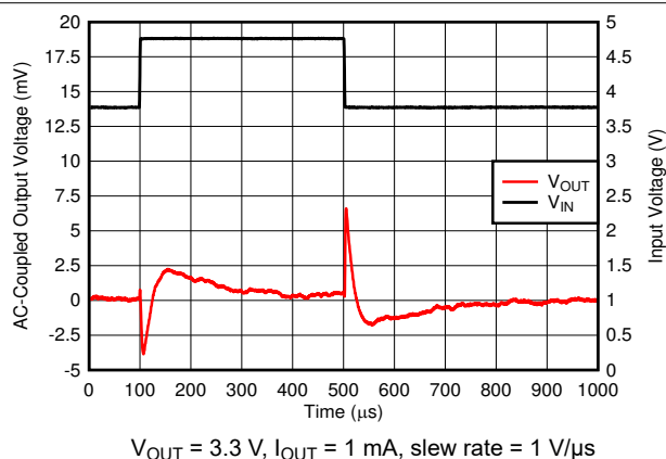
FIG 6-24. Line Transient
