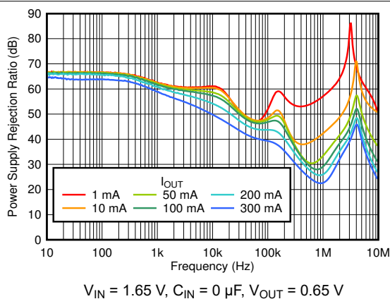
FIG 6-65. PSRR vs Frequency and I_{OUT}
