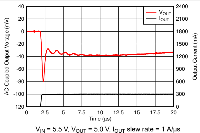
FIG 6-42. I_{OUT} Transient From 1 mA to 300 mA
