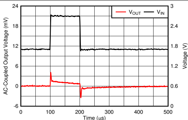
FIG 6-26. Line Transient
