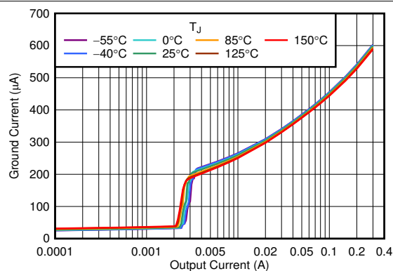
FIG 6-14. I_{GND} vs I_{OUT}
