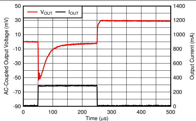
FIG 6-57. Load Transient
