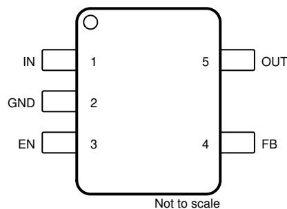
✎ 5-2. DBV Package (Adjustable), 5-Pin SOT-23, Top View
