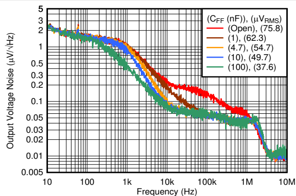
FIG 6-73. Output Noise vs Frequency and C_{FF}
