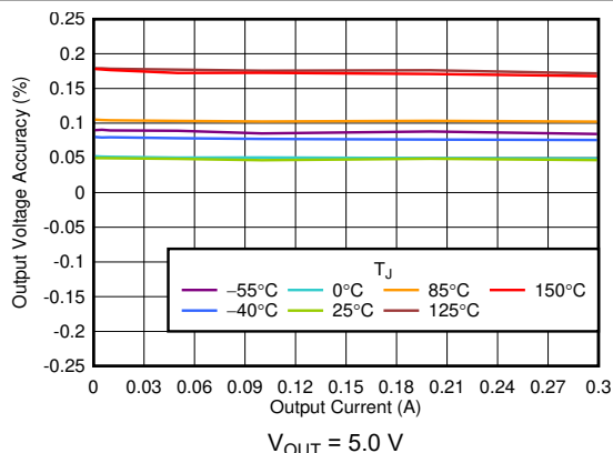
6-5. Output Accuracy vs I_{\text{OUT}}
