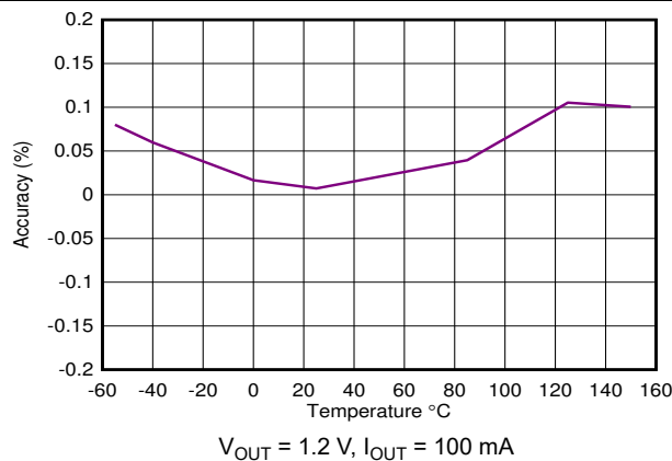
FIG 6-9. Accuracy vs Temperature
