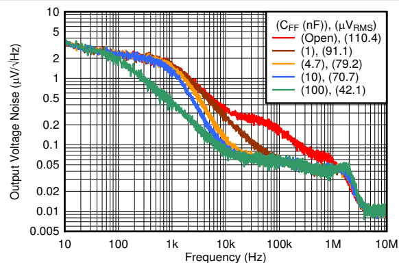
FIG 6-74. Output Noise vs Frequency and C_{FF}
