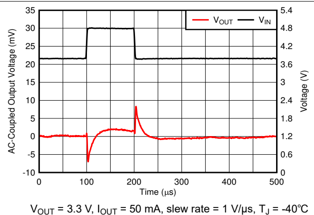
FIG 6-36. Line Transient
