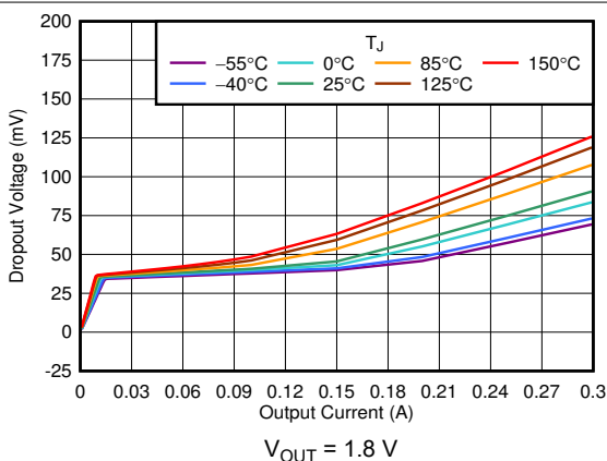
FIG 6-11. Dropout Voltage vs I_{OUT}
