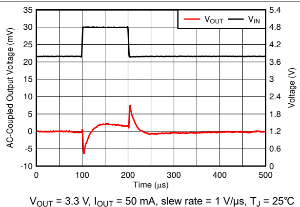
FIG 6-35. Line Transient
