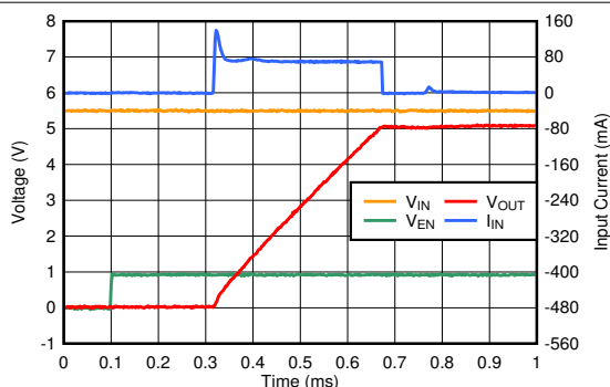
FIG 6-75. Start-Up Inrush Current With C_{OUT} = 1\text{ }\mu\text{F}
