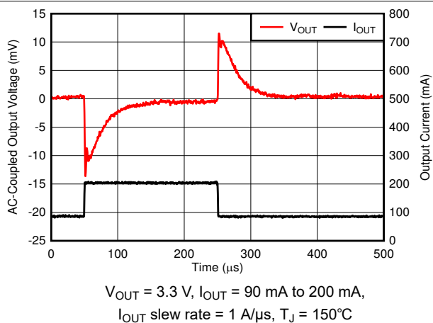
FIG 6-64. Load Transient
