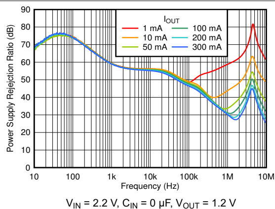
FIG 6-66. PSRR vs Frequency and I_{OUT}
