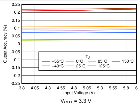
6-4. Output Accuracy vs V_{\text{IN}}
