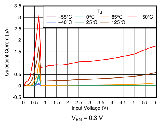
FIG 6-18. I_{SHDN} vs V_{IN}
