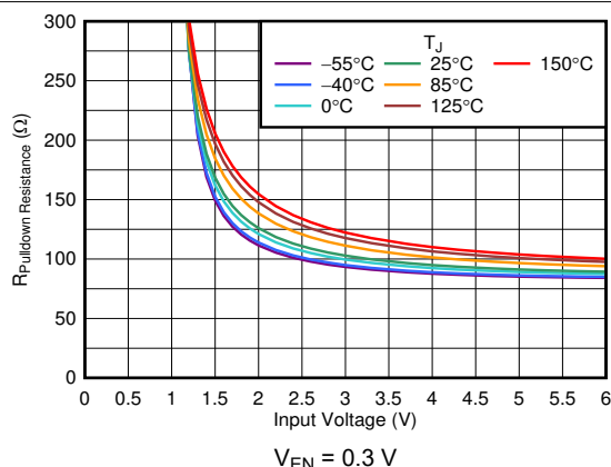
FIG 6-19. Pulldown Resistor ( R_{Pulldown} ) vs V_{IN}
