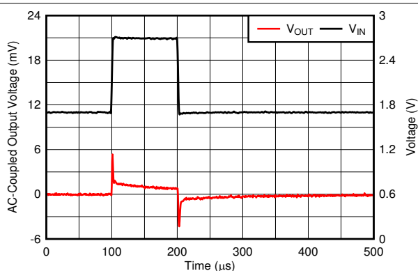
FIG 6-28. Line Transient
