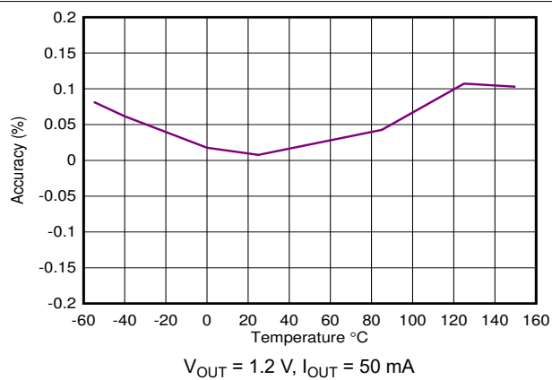
FIG 6-8. Accuracy vs Temperature
