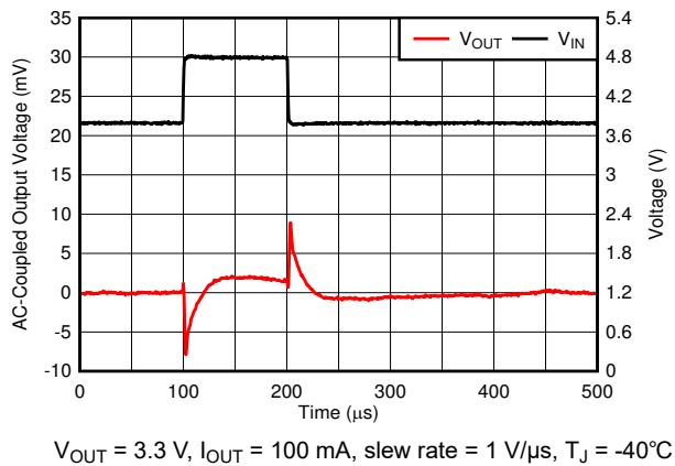
FIG 6-39. Line Transient
