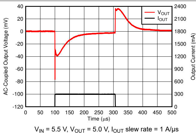
FIG 6-41. I_{OUT} Transient From 1 mA to 300 mA
