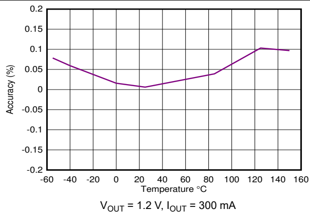
FIG 6-10. Accuracy vs Temperature
