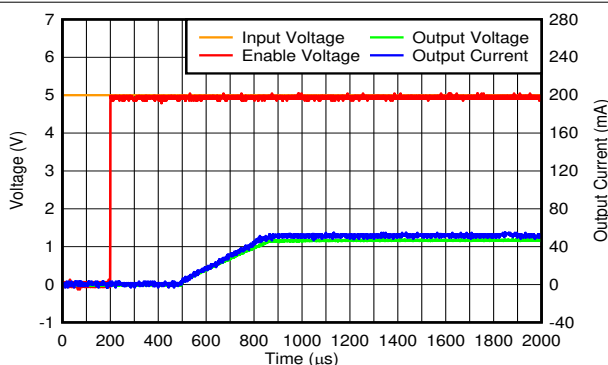
FIG 6-76. Start-Up Inrush Current With C_{OUT} = 1\text{ }\mu\text{F}
