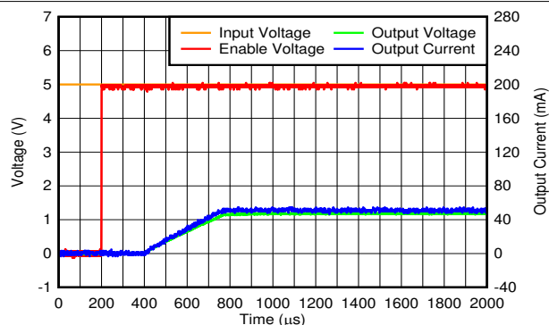
FIG 6-79. Start Up at 25^\circ\text{C}
