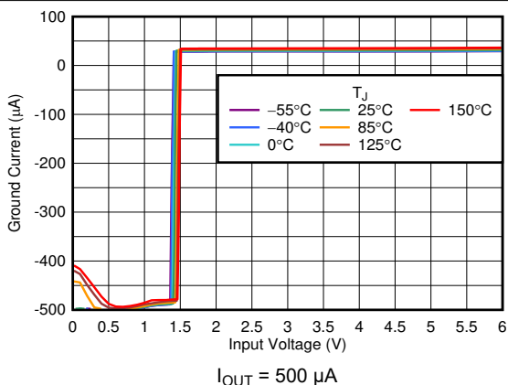
FIG 6-15. I_{GND} vs V_{IN}
