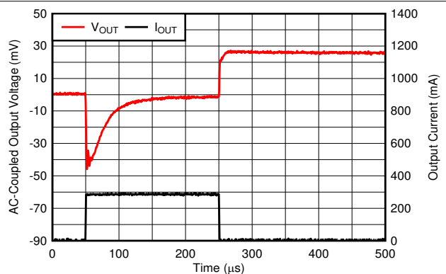
FIG 6-58. Load Transient
