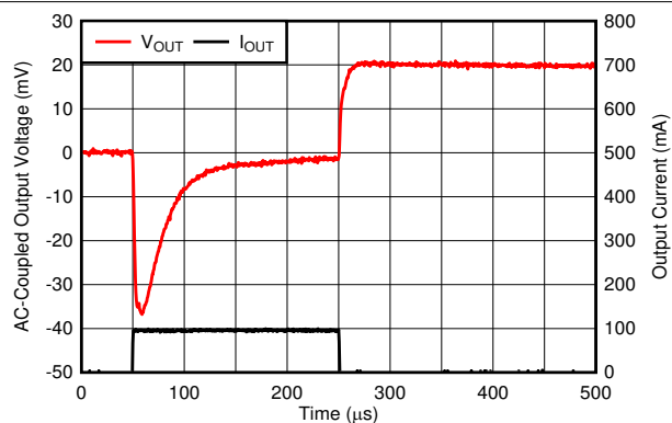
FIG 6-56. Load Transient
