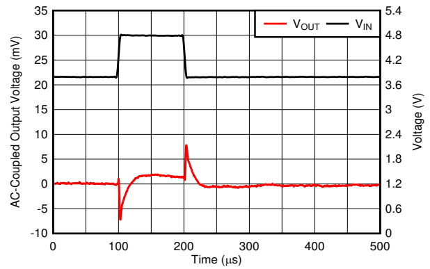
FIG 6-38. Line Transient
