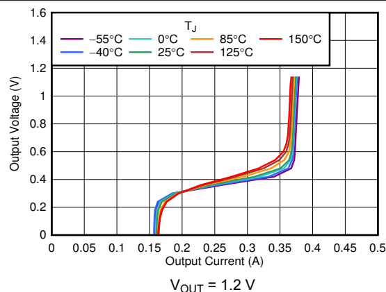
FIG 6-22. Foldback Current Limit vs I_{OUT} and Temperature
