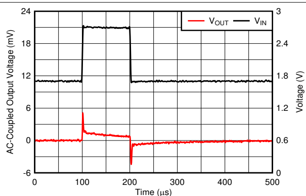
FIG 6-27. Line Transient
