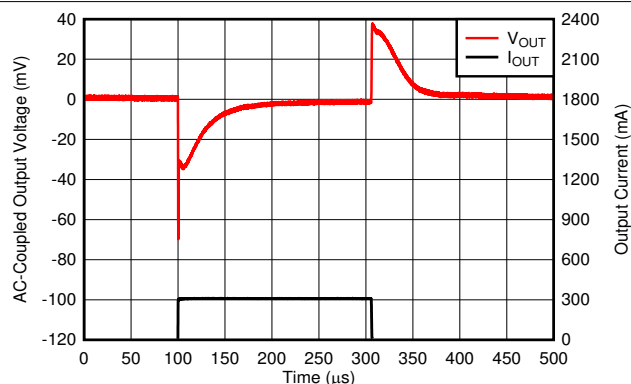
FIG 6-44. I_{OUT} Transient From 1 mA to 300 mA
