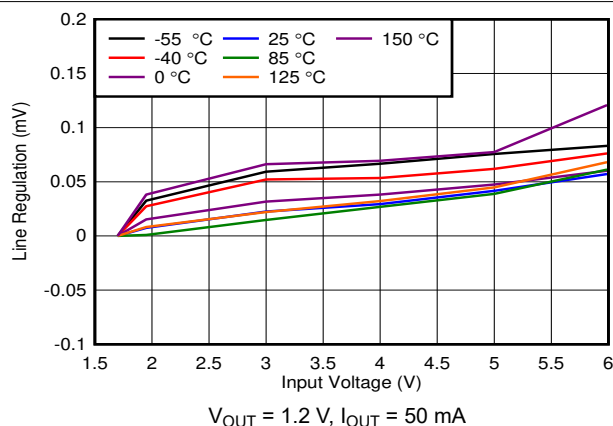
FIG 6-7. 50-mA Line Regulation
