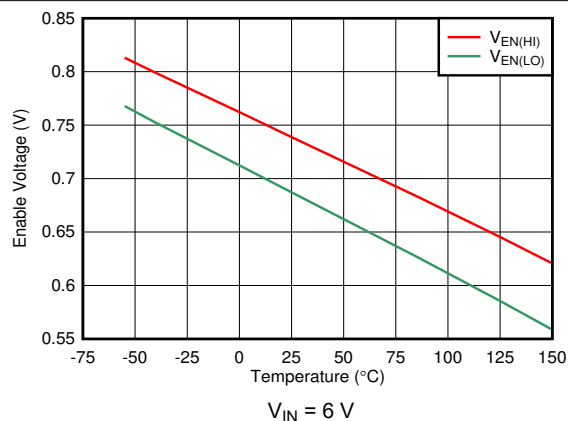
FIG 6-21. V_{EN(HI)} and V_{EN(LO)} Thresholds vs Temperature
