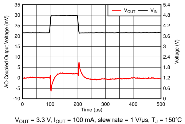
FIG 6-40. Line Transient
