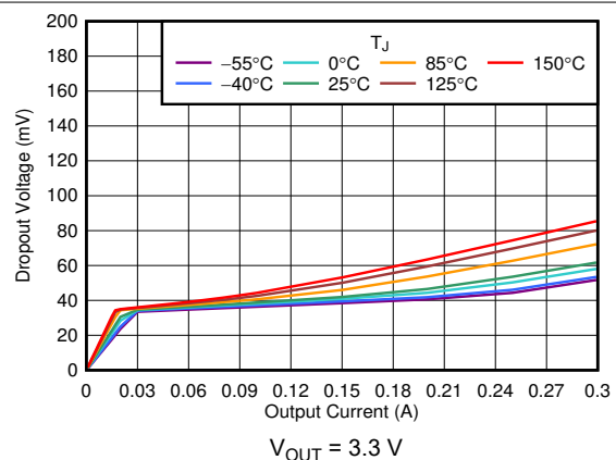
FIG 6-12. Dropout Voltage vs I_{OUT}
