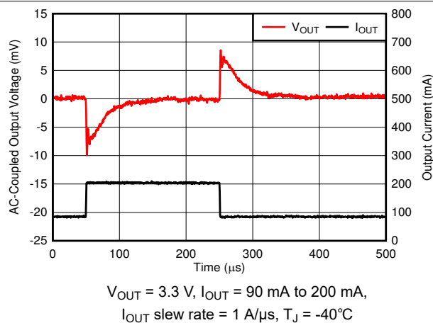
FIG 6-63. Load Transient
