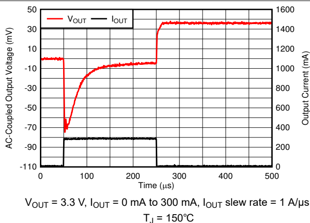
FIG 6-61. Load Transient
