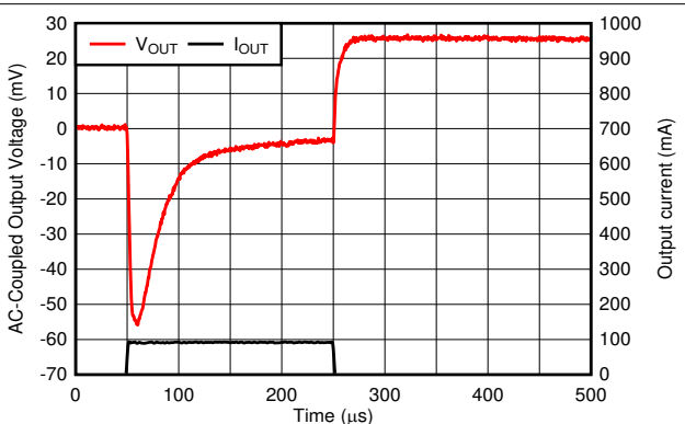
FIG 6-56. Load Transient
