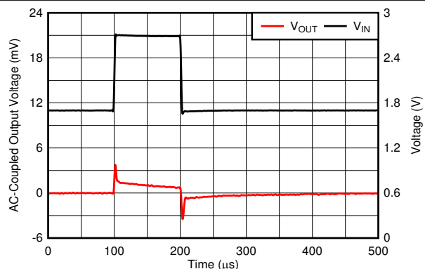
FIG 6-25. Line Transient
