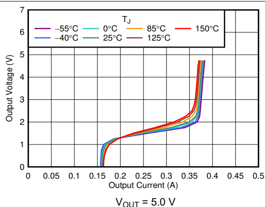
FIG 6-23. Foldback Current Limit vs I_{OUT} and Temperature
