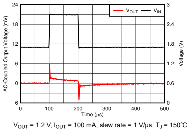
FIG 6-31. Line Transient
