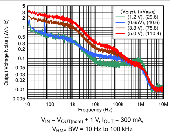
Figure 6-72. Output Noise vs Frequency and V_{OUT}
