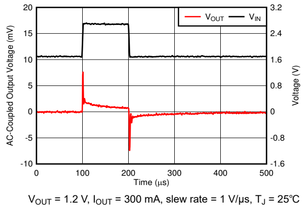
FIG 6-32. Line Transient
