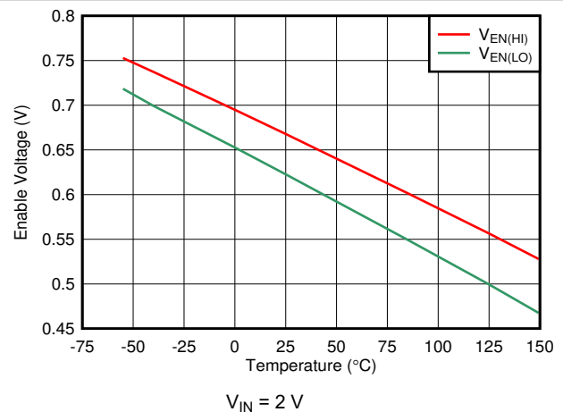
FIG 6-12. V_{EN(HI)} and V_{EV(LO)} Threshold vs Temperature
