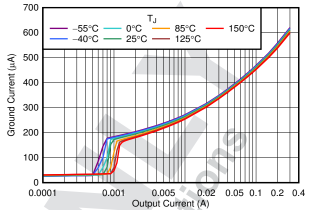
FIG 6-8. I_{GND} vs I_{OUT}
