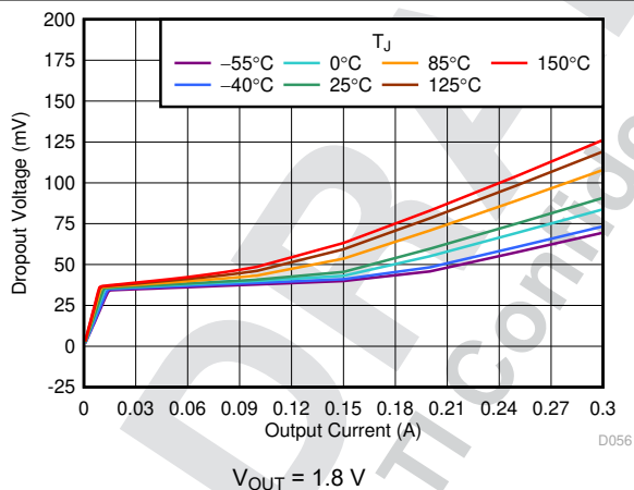
6-5. Dropout Voltage vs I_{OUT}
