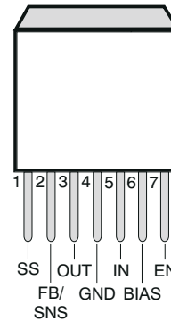
図 4-2. KTW Package, 7-Pin DDPak/TO-263 (Top View, Legacy Chip)
