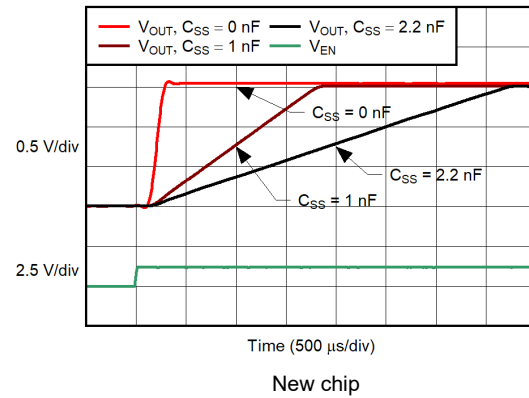
图 5-38. Turn-On Response
