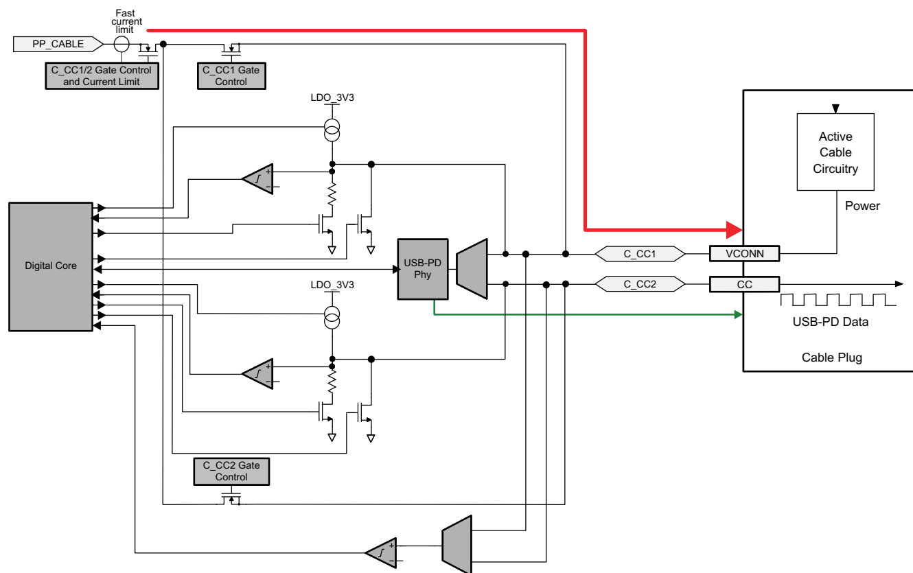
FIG 9-30. Port C_CC1 and C_CC2 Reverse Orientation Power from PP_CABLE
