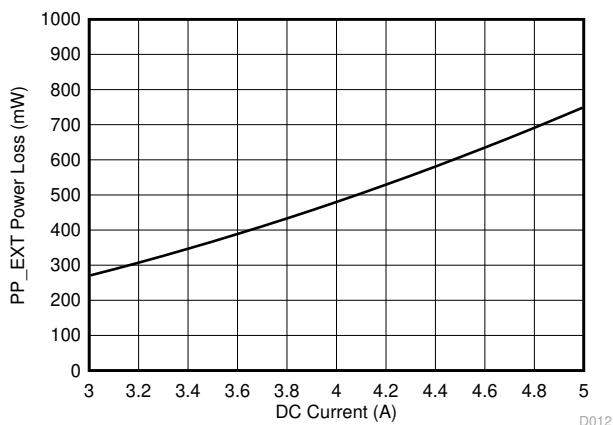
FIG 10-2. PP_EXT Power Loss
