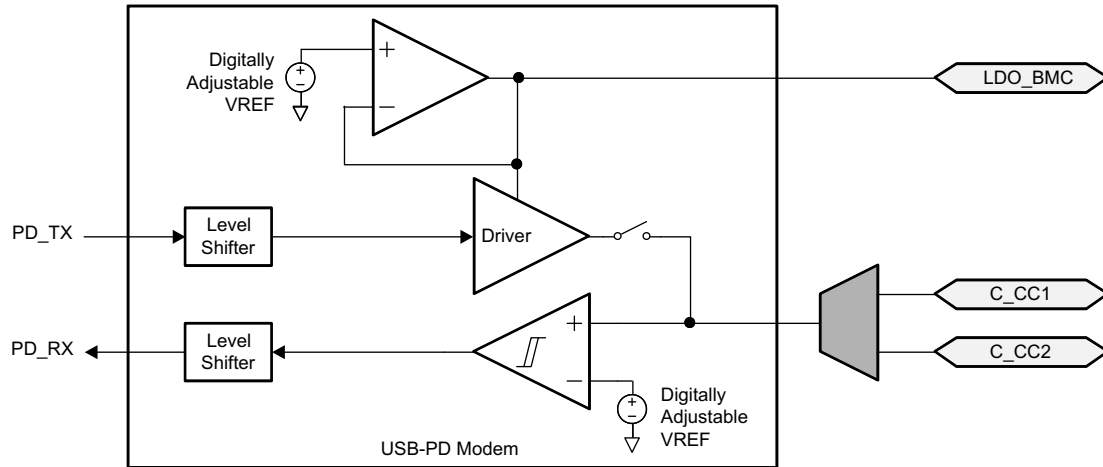
FIG 9-5. USB-PD BMC TX/Rx Block Diagram
