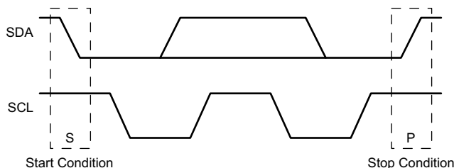
✎ 9-62. I 2 C Definition of Start and Stop Conditions
