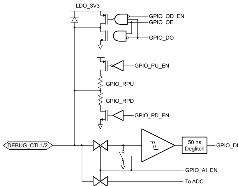
FIG 9-46. IOBUF_GPIOLSI2C (General GPIO) I/O with I 2 C Deglitch
