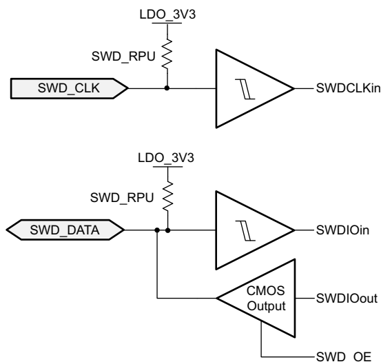
9-53. IOBUF_GPIOHSSWD
