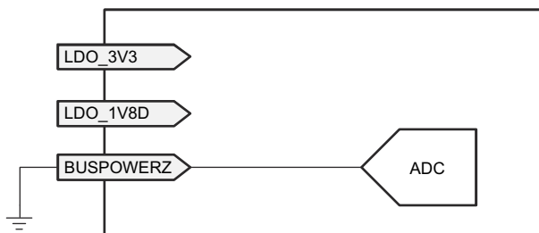
FIG 9-24. BUSPOWERZ Configured with PP_EXT as Input Power Path
