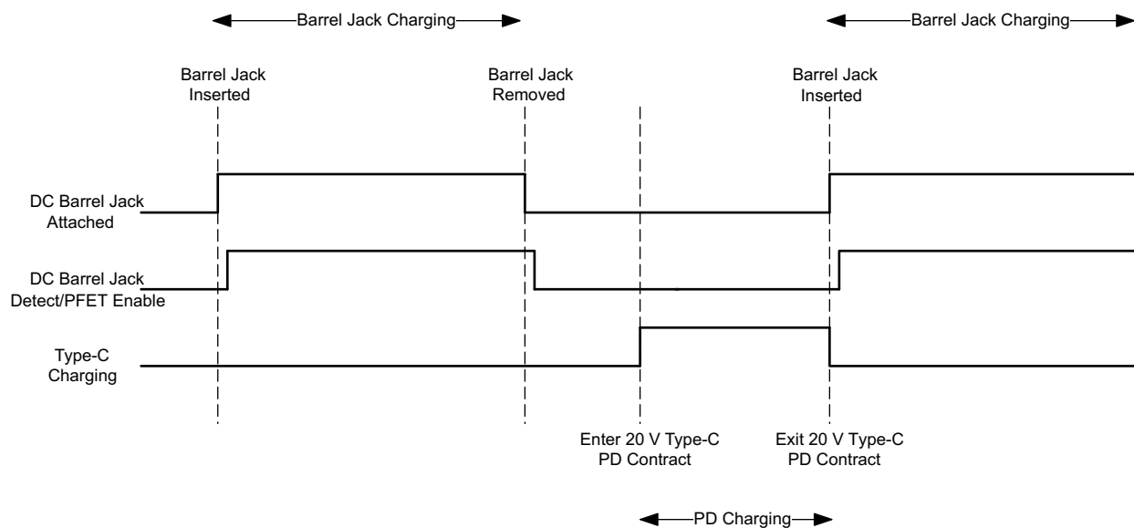
FIG 10-6. DC Barrel Jack and Type-C PD Charging Hand-Off
