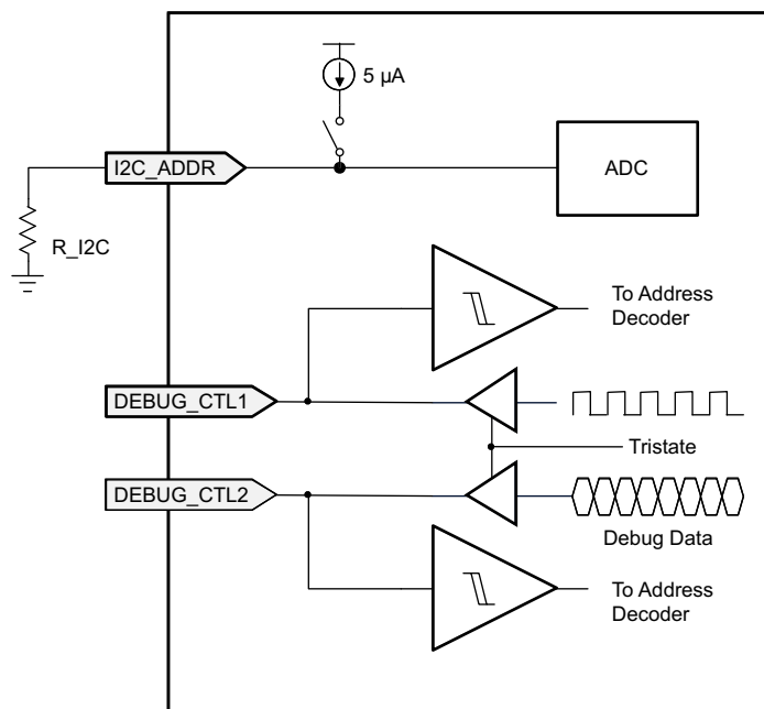
9-68. I 2 C Address Decode
