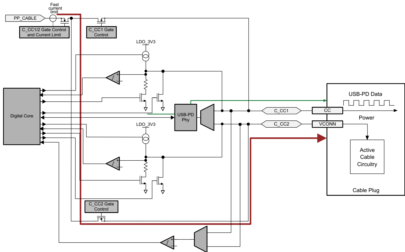
9-29. Port C_CC1 and C_CC2 Normal Orientation Power from PP_CABLE
