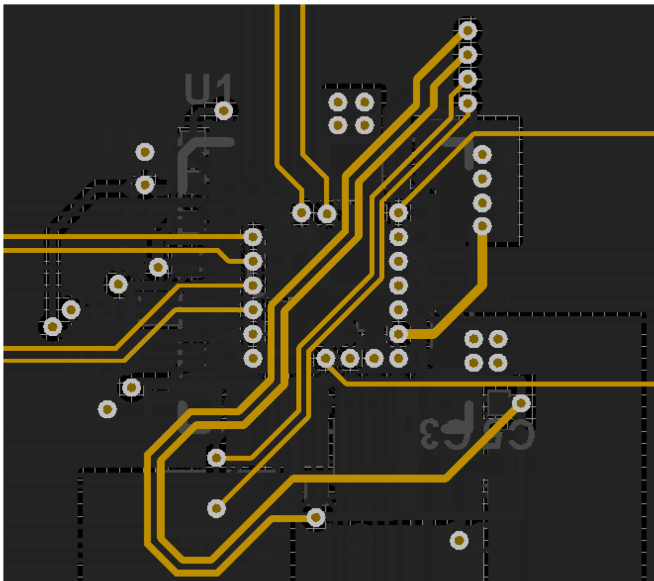
図 12-18. Final Routing (Inner Signal Layer)
