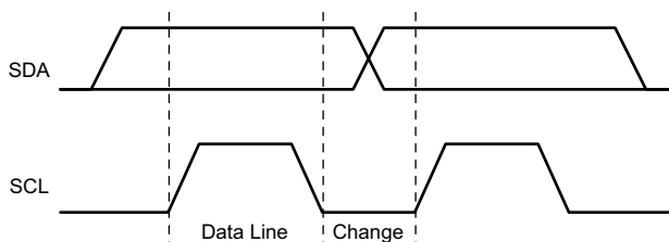
✎ 9-63. I 2 C Bit Transfer
