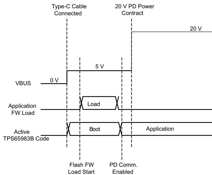
FIG 10-7. Primary TPS65983B Dead Battery Sequence
