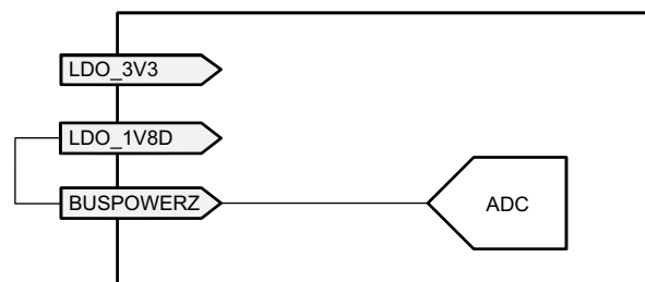
FIG 9-23. BUSPOWERZ Configured with PP_HV as Input Power Path
