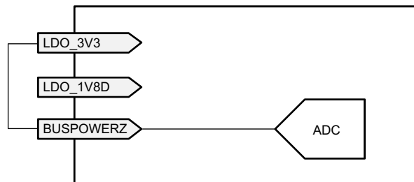
FIG 9-22. BUSPOWERZ Configured to Disable Power from VBUS
