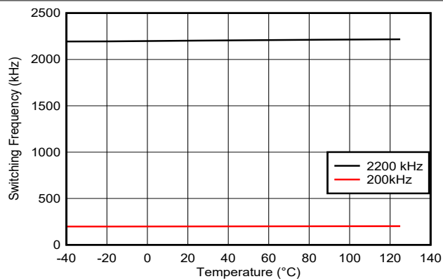
FIG 6-16. Switching Frequency vs Temperature
