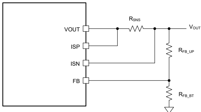
7-5. Output Voltage Setting
