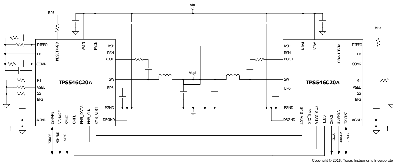
☒ 23. 2-Phase Application
