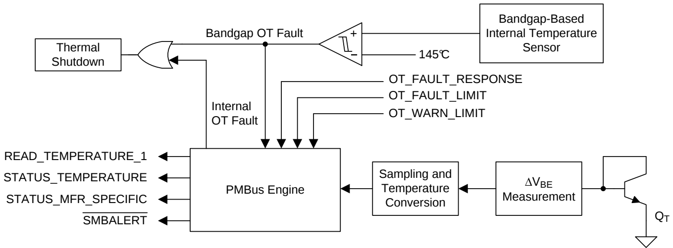
✎ 33. Overtemperature Protection
