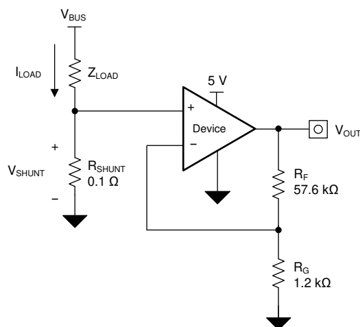
図 9-1. TLV904x in a Low-Side, Current-Sensing Application
